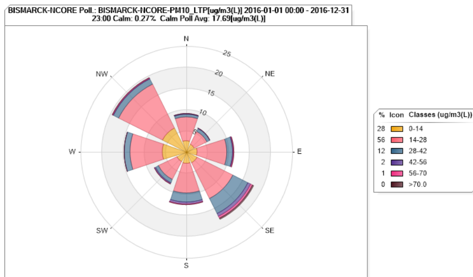
Figure 34. Bismarck PM 10 Pollution Rose for 2016
