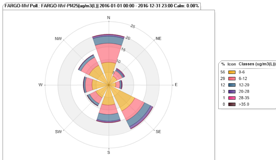
Figure 46. Fargo PM 2.5 Pollution Rose for 2016
