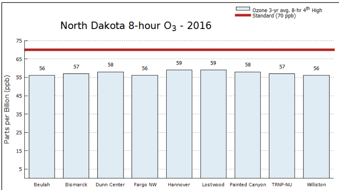
Figure 10. Ozone Concentrations compared to the 8-hour Standard
