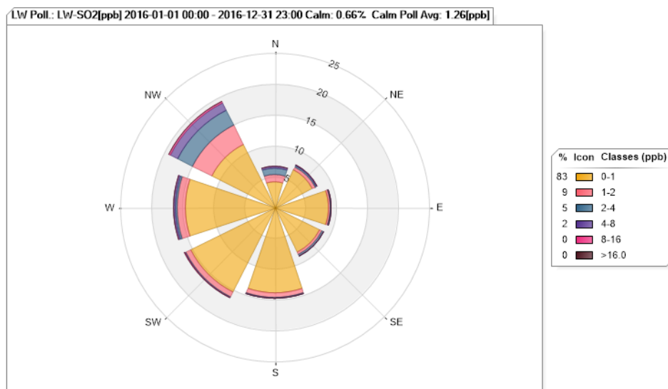
Figure 59. Lostwood SO 2 Pollution Rose for 2016
