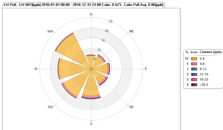
Figure 60. Lostwood NH 3 Pollution Rose for 2016
