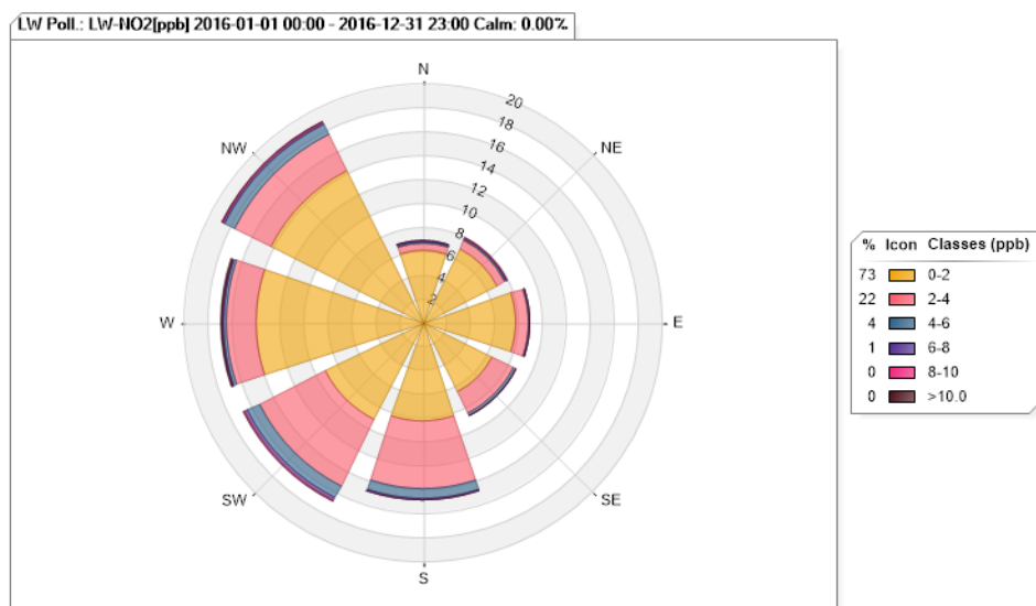
Figure 55. Lostwood NO 2 Pollution Rose for 2016
