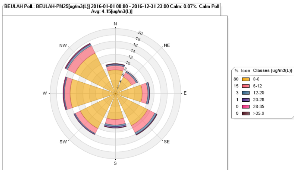
Figure 28. Beulah PM 2.5 Pollution Rose for 2016
