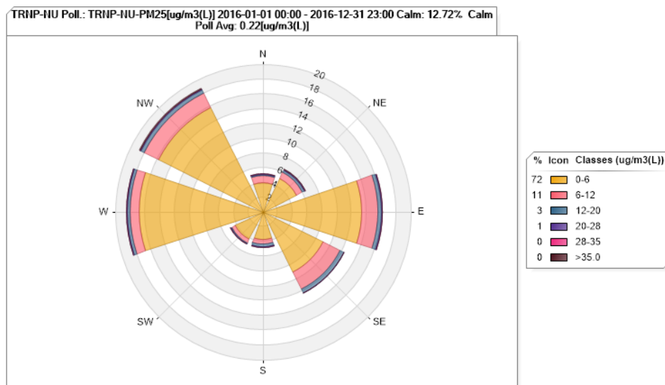
Figure 69. TRNP – North Unit PM 2.5 Pollution Rose for 2016
