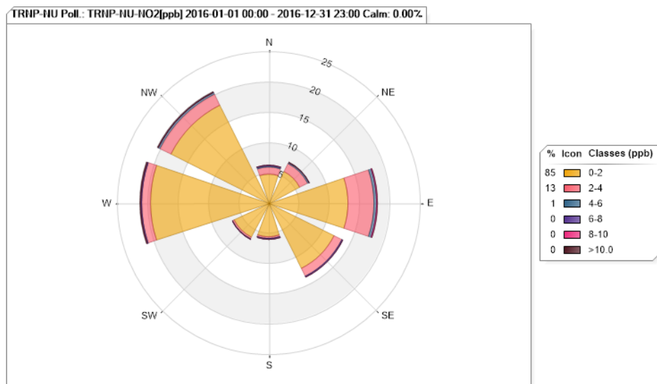
Figure 66. TRNP – North Unit NO 2 Pollution Rose for 2016
