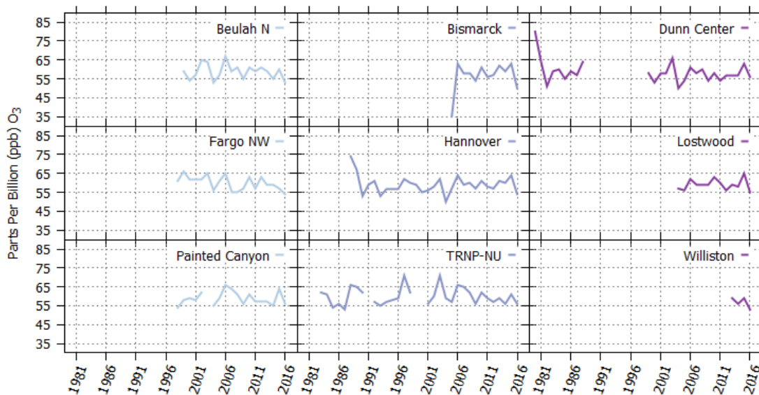
Figure 11. Annual 4 th Highest 8-HR Ozone Concentrations
