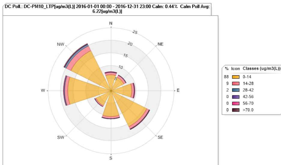
Figure 39. Dunn Center PM 10 Pollution Rose for 2016
