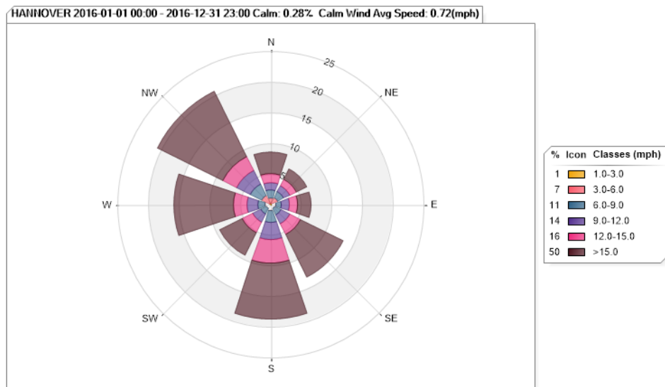
Figure 48. Hannover Wind Rose for 2016
