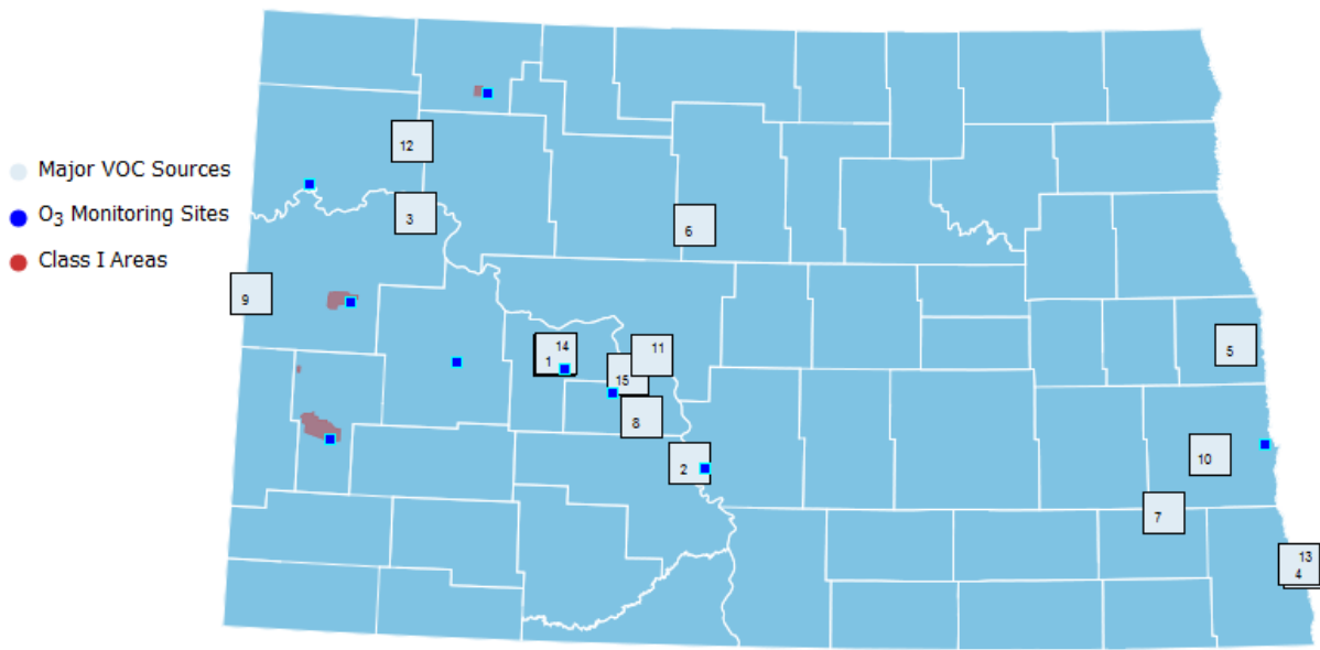
Figure 9. Major VOC Sources in 2016
