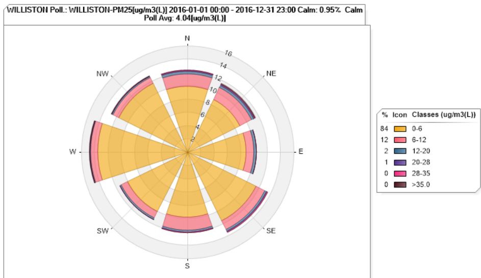
Figure 74. Williston PM 2.5 Pollution Rose for 2016
