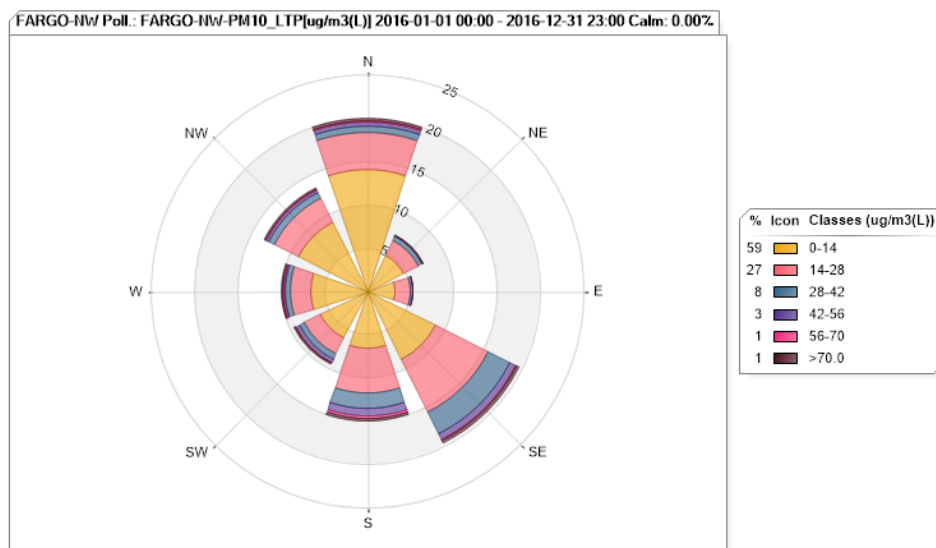
Figure 45. Fargo PM 10 Pollution Rose for 2016
