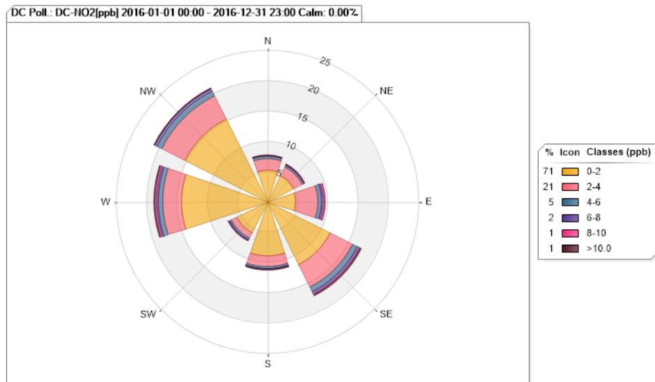
Figure 37. Dunn Center NO 2 Pollution Rose for 2016
