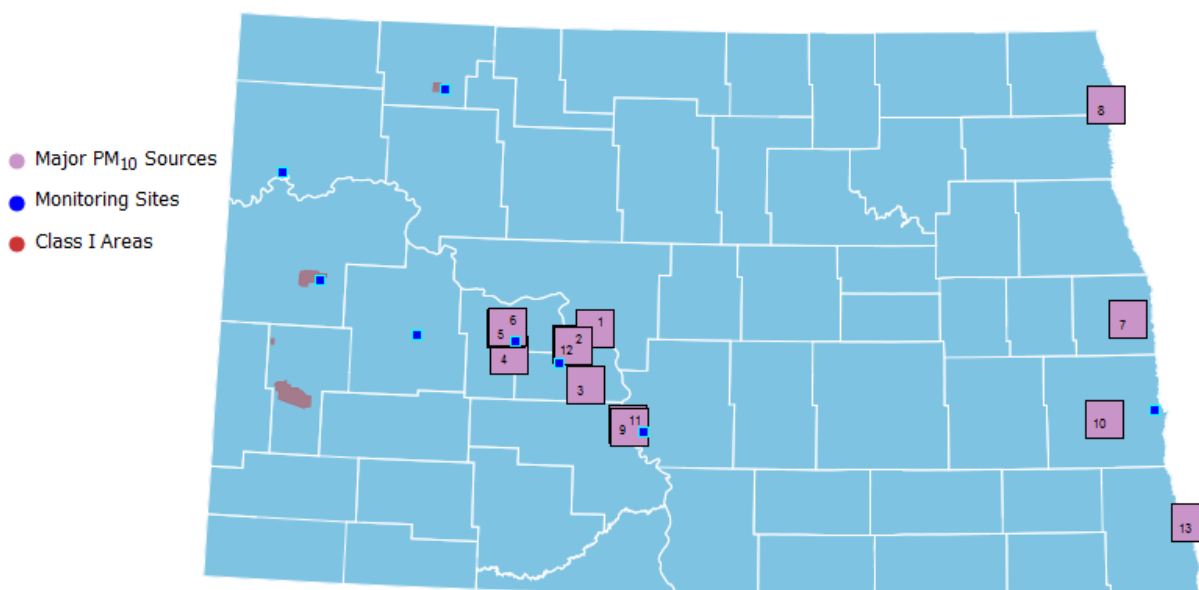
Figure 12. Major PM 10 Sources in 2016
