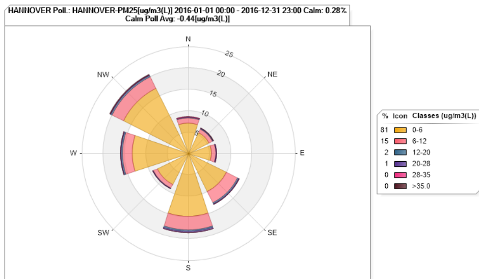
Figure 52. Hannover PM 2.5 Pollution Rose for 2016
