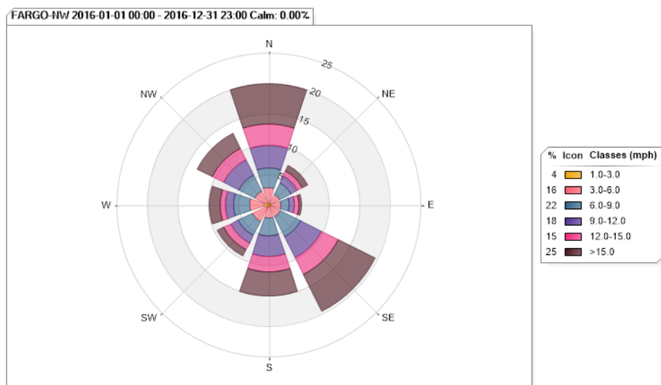
Figure 42. Fargo Wind Rose for 2016
