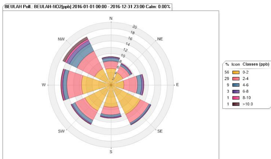
Figure 25. Beulah NO 2 Pollution Rose for 2016
