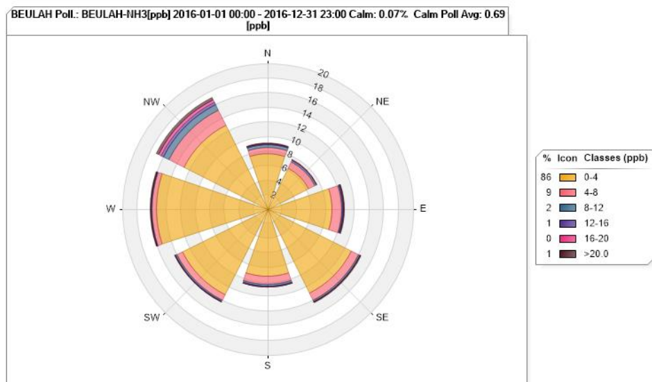
Figure 30. Beulah NH 3 Pollution Rose for 2016
