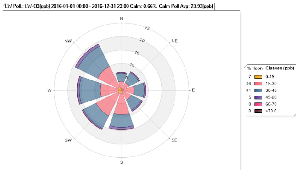
Figure 56. Lostwood O 3 Pollution Rose for 2016
