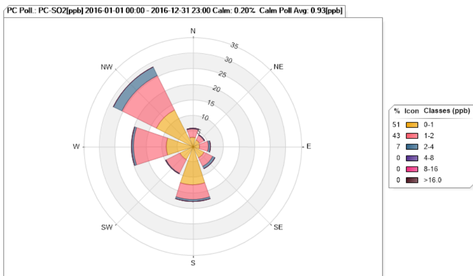
Figure 64. Painted Canyon SO 2 Pollution Rose for 2016
