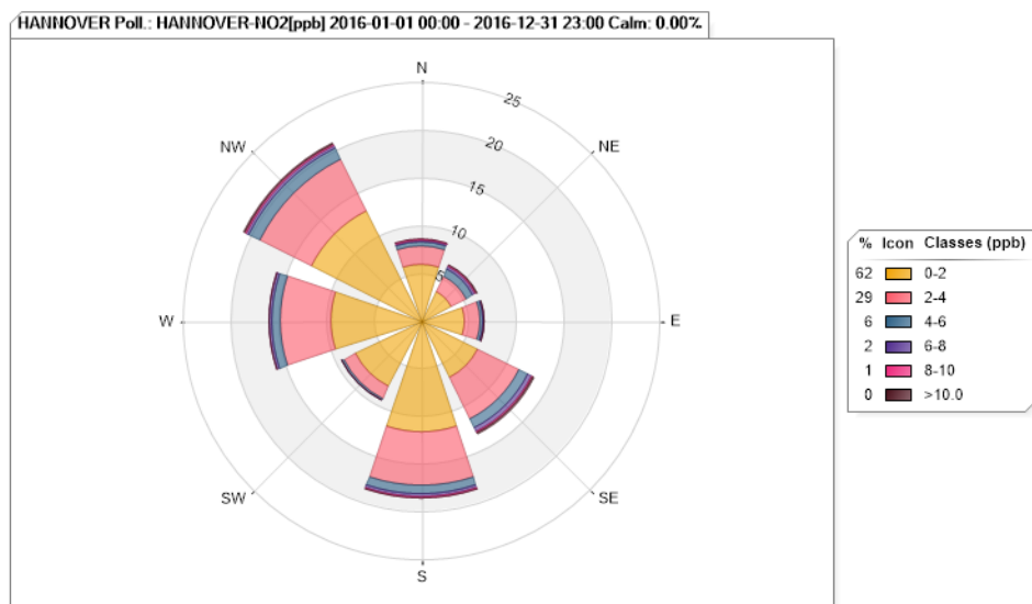
Figure 49. Hannover NO 2 Pollution Rose for 2016
