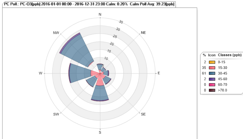
Figure 62. Painted Canyon O 3 Pollution Rose for 2016
