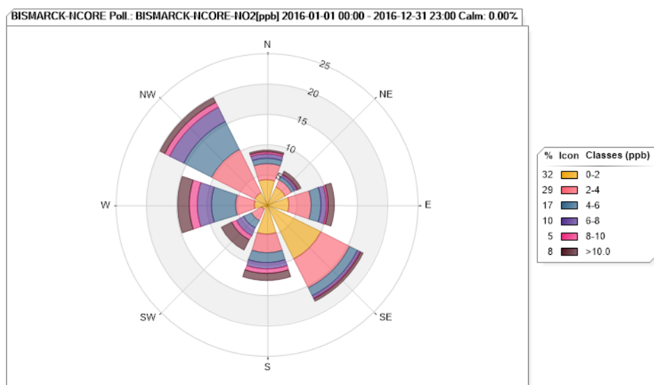
Figure 32. Bismarck NO 2 Pollution Rose for 2016
