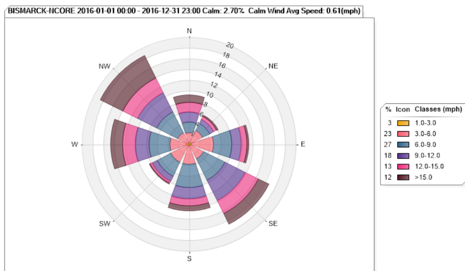
Figure 31. Bismarck Wind Rose for 2016
