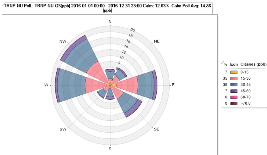
Figure 67. TRNP – North Unit O 3 Pollution Rose for 2016
