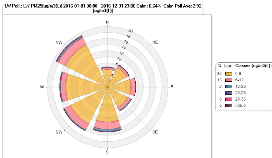
Figure 58. Lostwood PM 2.5 Pollution Rose for 2016
