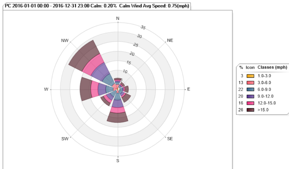
Figure 61. Painted Canyon Wind Rose for 2016
