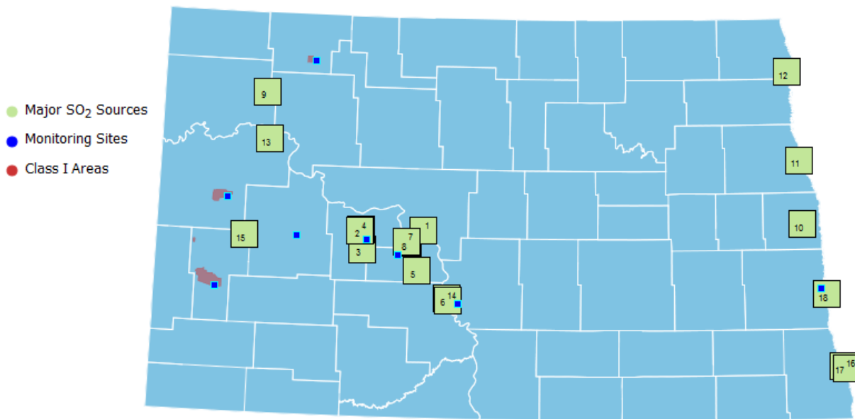
Figure 17. Major Sulfur Dioxide Sources in 2016
