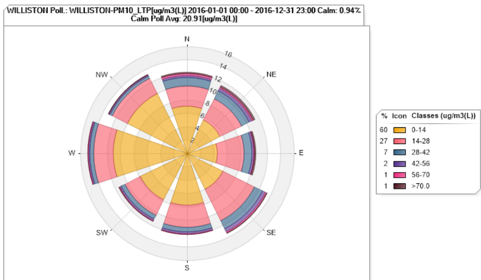
Figure 73. Williston PM 10 Pollution Rose for 2016
