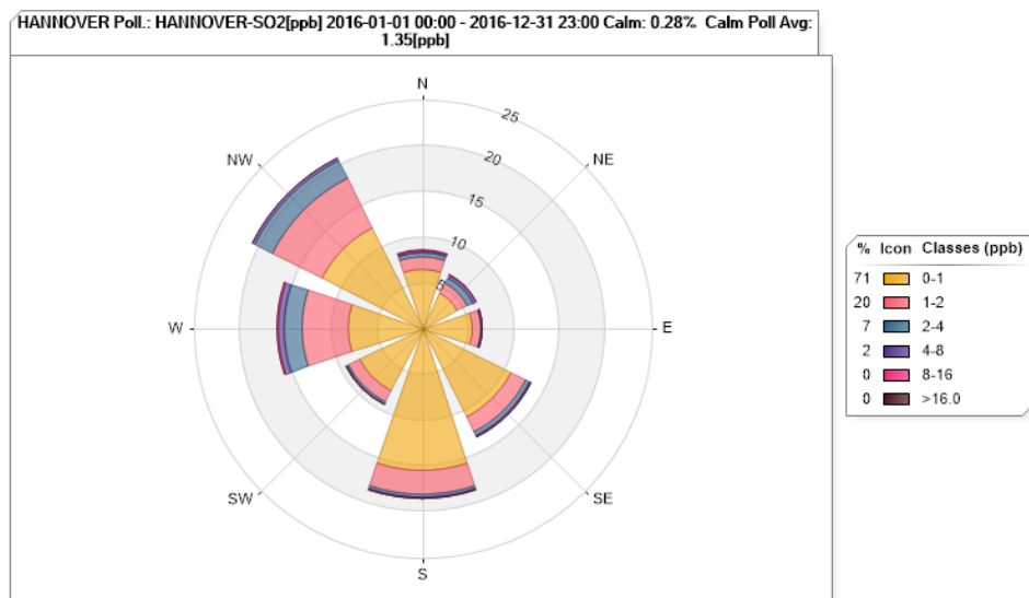
Figure 53. Hannover SO 2 Pollution Rose for 2016
