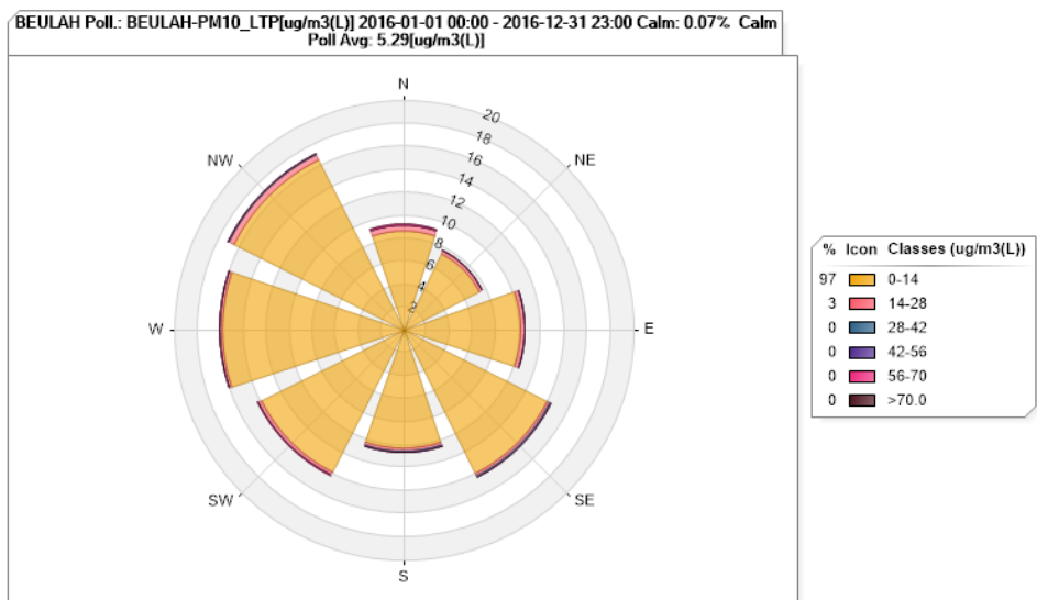
Figure 27. Beulah PM 10 Pollution Rose for 2016
