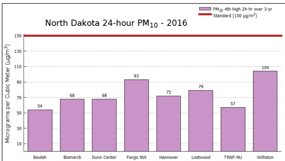
Figure 13. PM 10 Concentrations Compared to the 24-hour Standard 17
