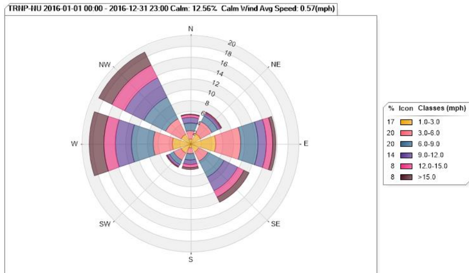
Figure 65. TRNP – North Unit Wind Rose for 2016
