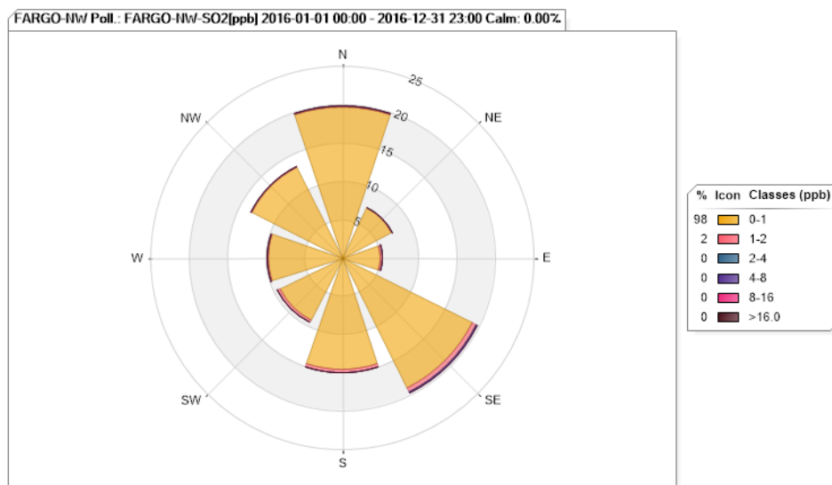
Figure 47. Fargo SO 2 Pollution Rose for 2016
