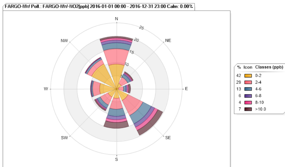
Figure 43. Fargo NO 2 Pollution Rose for 2016
