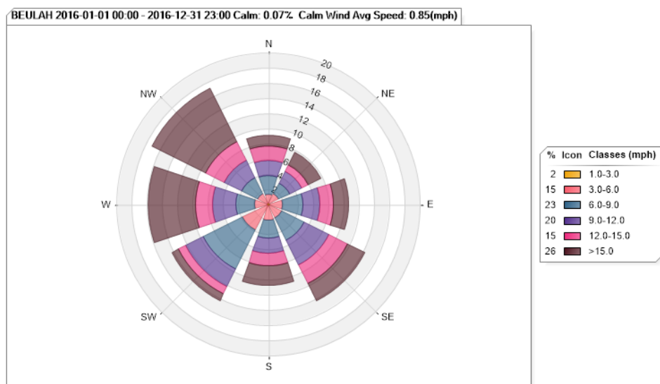
Figure 24. Beulah Wind Rose for 2016
