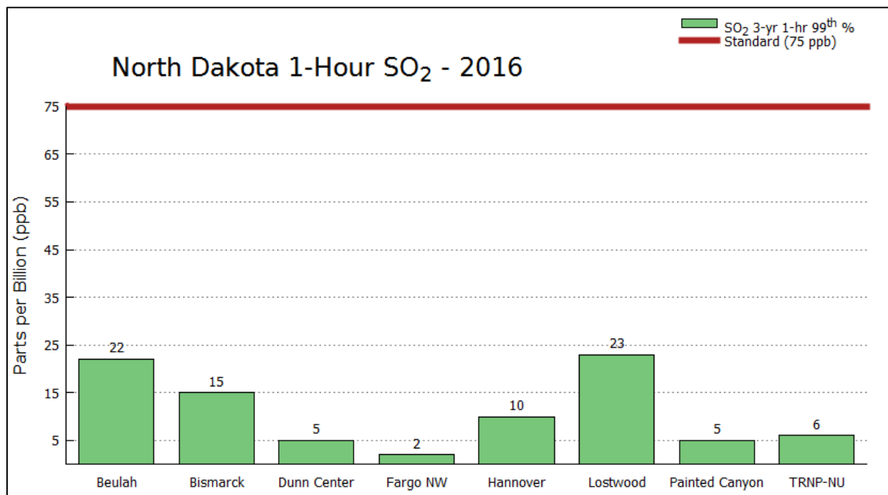
Figure 18. SO 2 Concentrations Compared to the 1-hour Standard
