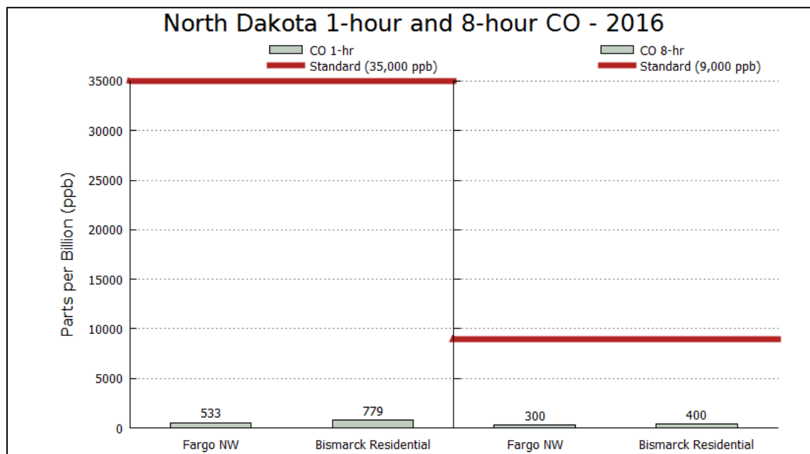
Figure 3. CO Concentrations (2 nd high) Compared to the 1-hour and 8-hour Standards (Partial year)
