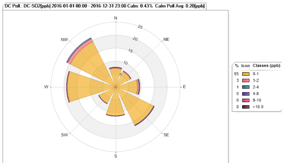
Figure 41. Dunn Center SO 2 Pollution Rose for 2016
