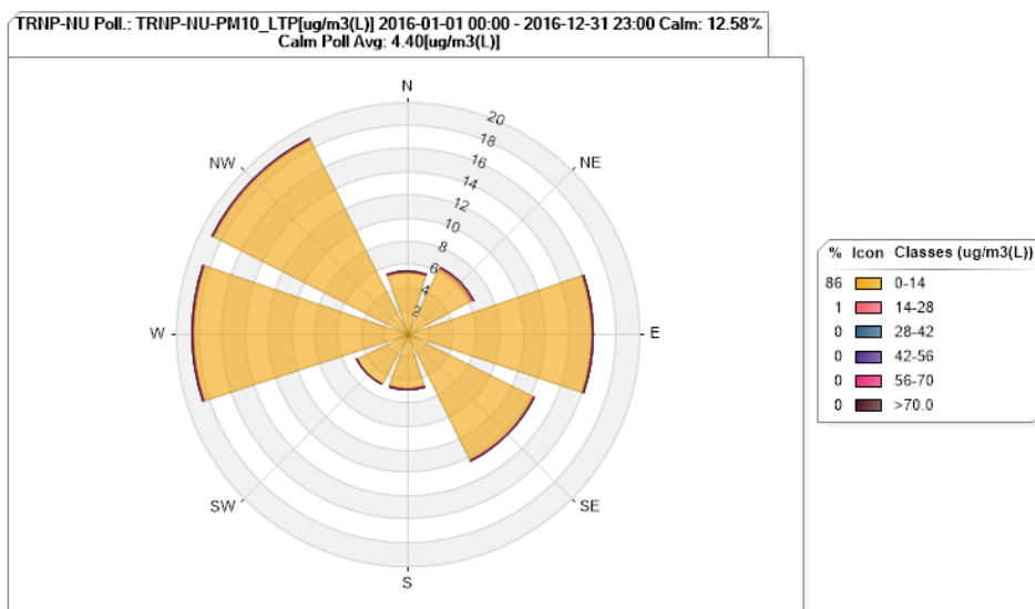
Figure 68. TRNP – North Unit PM 10 Pollution Rose for 2016
