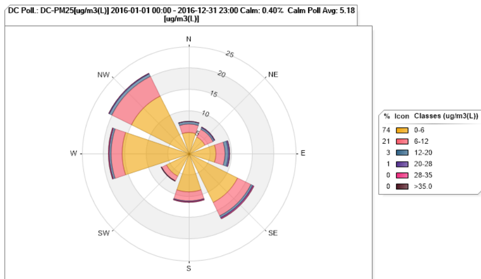
Figure 40. Dunn Center PM 2.5 Pollution Rose for 2016
