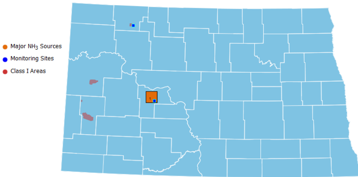
Figure 20. Major Ammonia Sources in 2016
