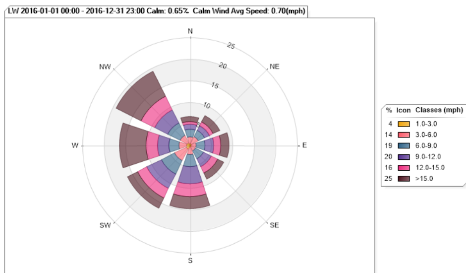
Figure 54. Lostwood Wind Rose for 2016
