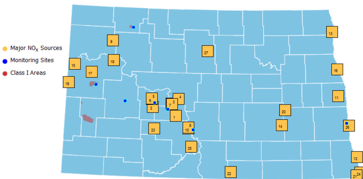
Figure 4. Major Oxides of Nitrogen Sources in 2016
