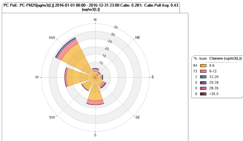
Figure 63. Painted Canyon PM 2.5 Pollution Rose for 2016
