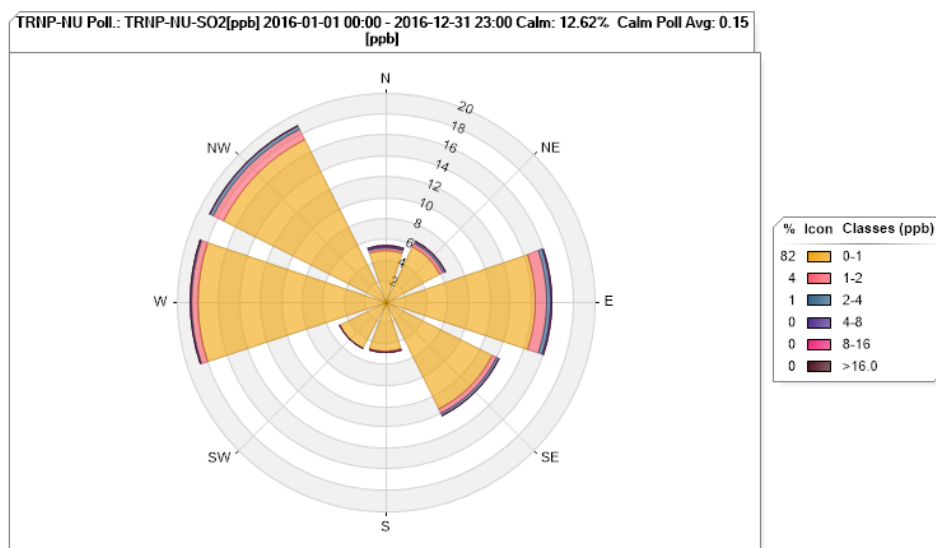
Figure 70. TRNP – North Unit SO 2 Pollution Rose for 2016
