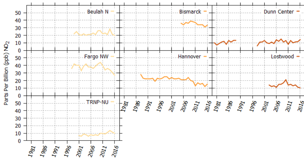
Figure 7. NO 2 98 th Percentile 1-Hour Concentrations
