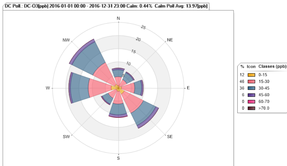
Figure 38. Dunn Center O 3 Pollution Rose for 2016
