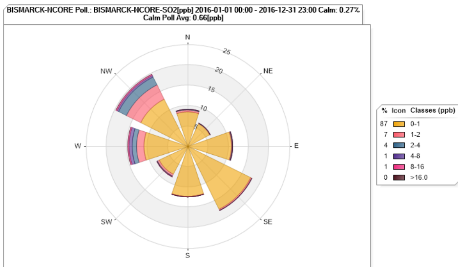
Figure 35. Bismarck SO 2 Pollution Rose for 2016
