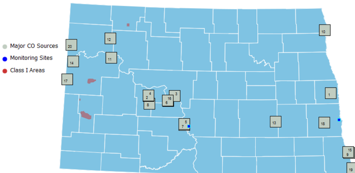
Figure 2. Major CO Sources in 2016 (Monitoring ended in Fargo and began in Bismarck during 2016)
