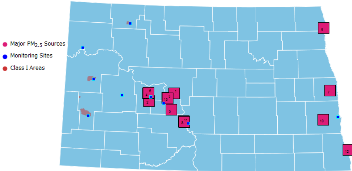
Figure 14 Major PM 2.5 Sources in 2016
