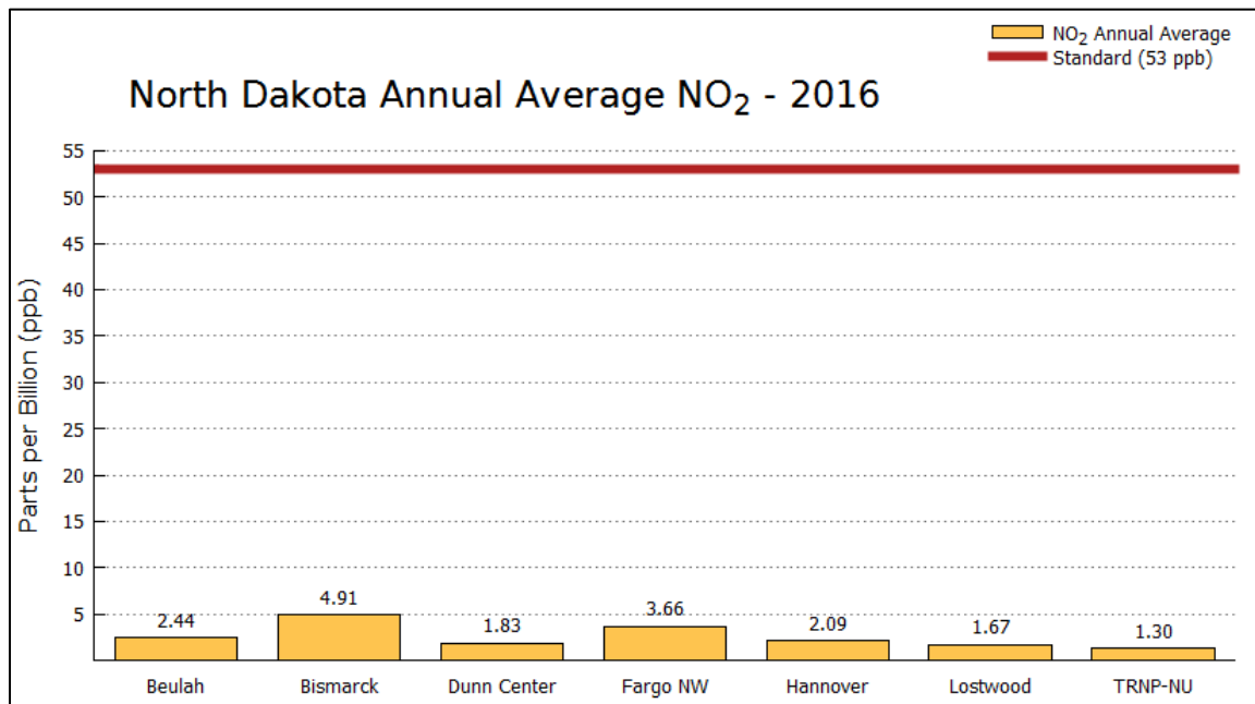
Figure 6. NO 2 Concentrations Compared to the Annual Standard
