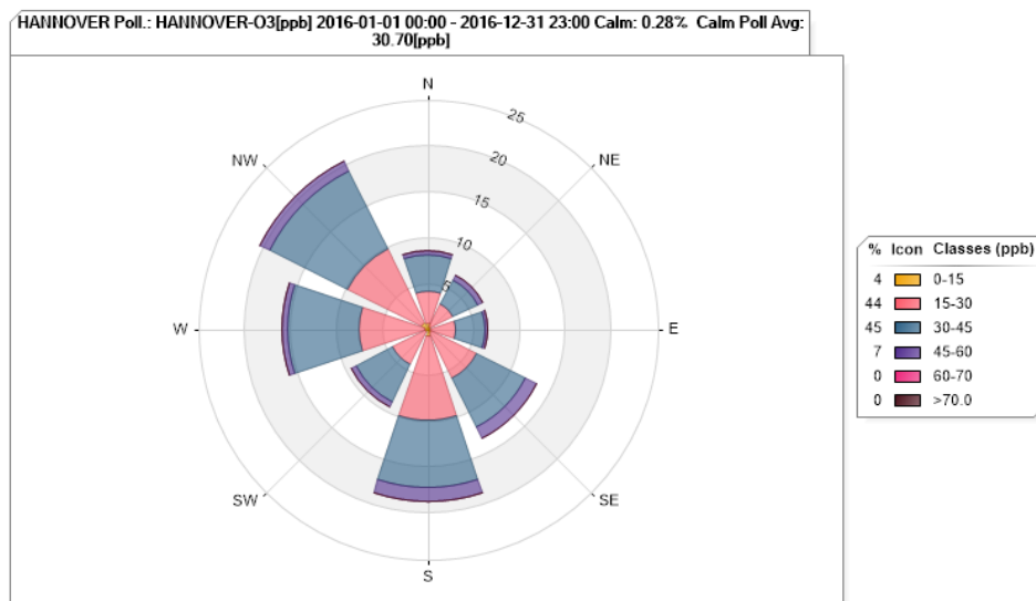
Figure 50. Hannover O 3 Pollution Rose for 2016
