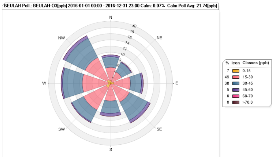
Figure 26. Beulah O 3 Pollution Rose for 2016
