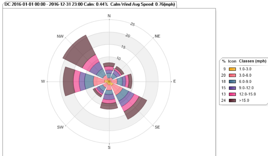
Figure 36. Dunn Center Wind Rose for 2016
