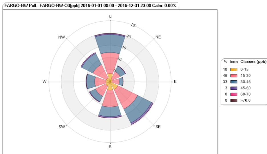
Figure 44. Fargo O 3 Pollution Rose for 2016
