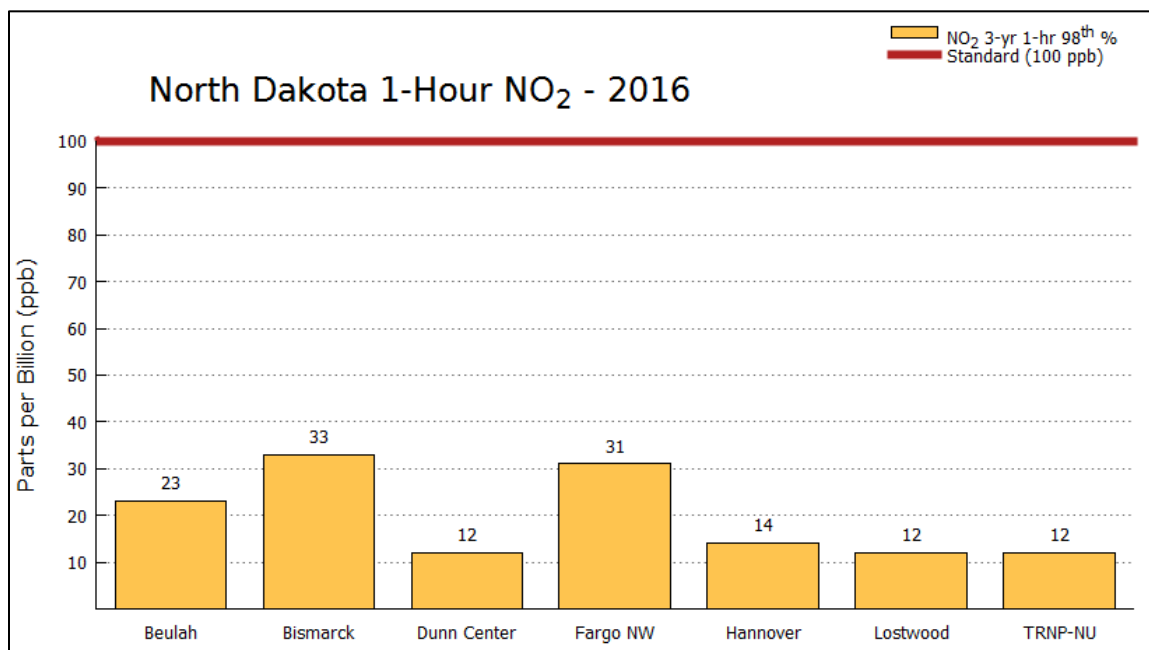
Figure 5. NO 2 Concentrations Compared to the 1-hour Standard
