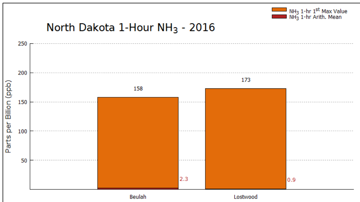
Figure 21. NH 3 Concentrations: Maximum Value and Arithmetic Mean
