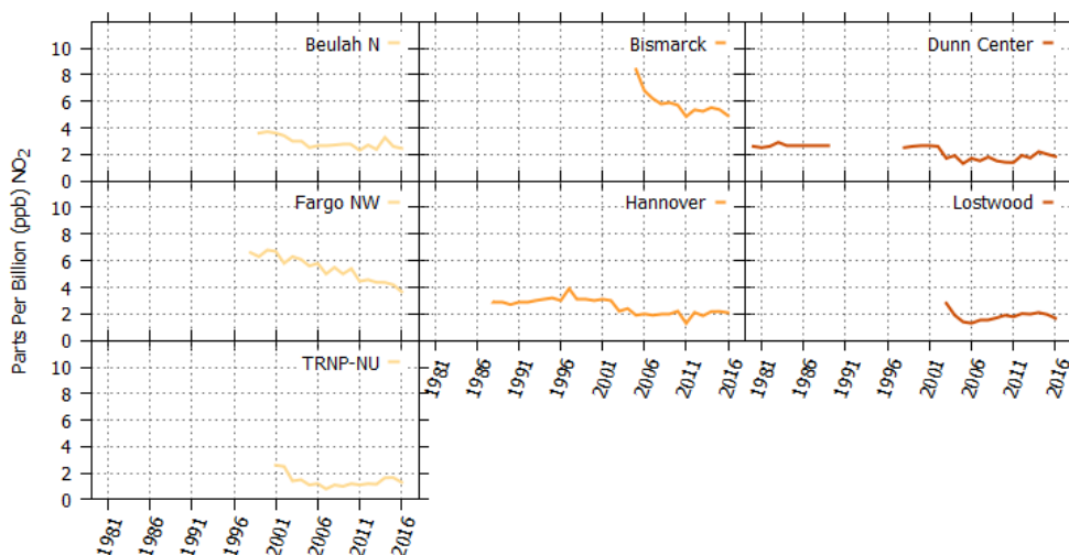
Figure 8. NO 2 Annual Average Concentrations
