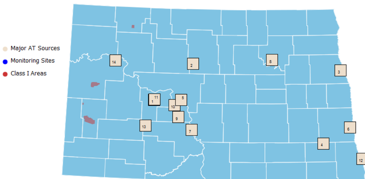
Figure 22. Major Air Toxics Sources in 2016
