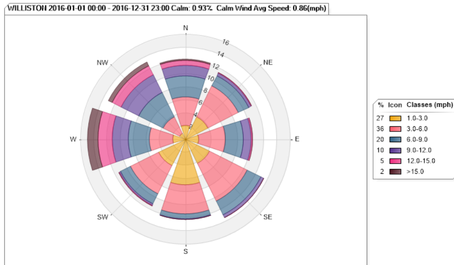
Figure 71. Williston Wind Rose for 2016
