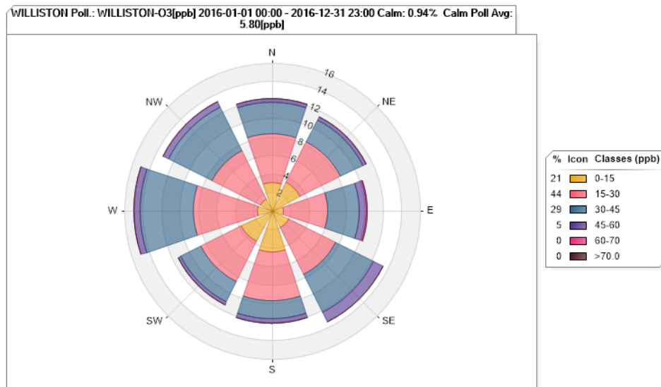
Figure 72. Williston O 3 Pollution Rose for 2016
