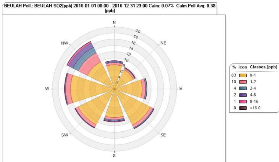
Figure 29. Beulah SO 2 Pollution Rose for 2016
