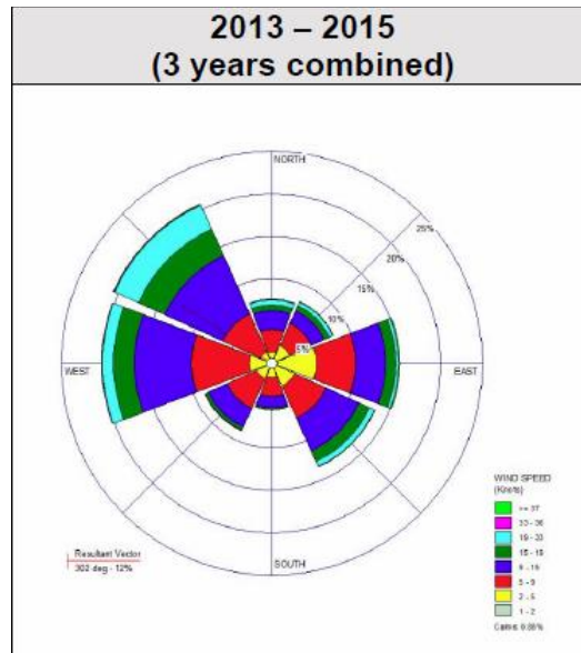
Figure 75. Tioga Gas Plant Wind Rose – Three Year Summary (Reproduced from Figure 14 of Hess modeling analysis report 23 )
