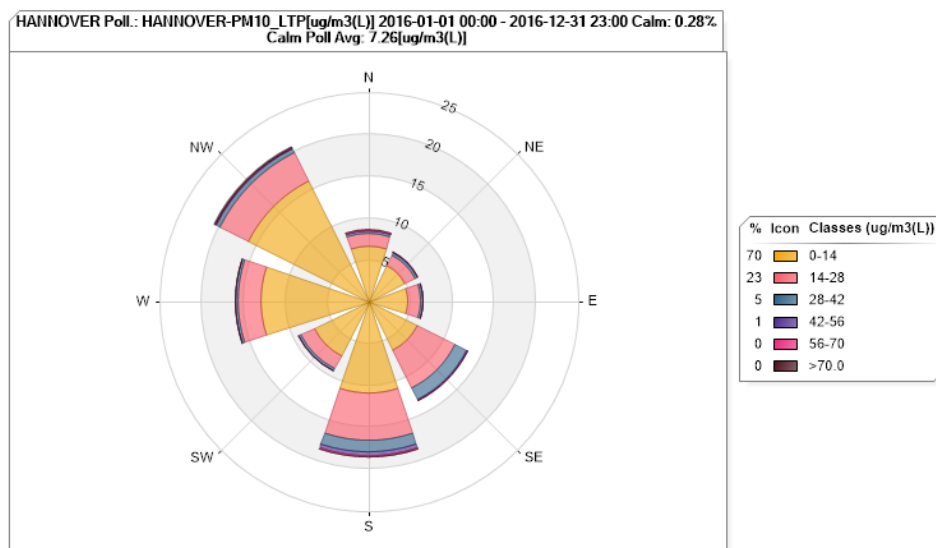
Figure 51. Hannover PM 10 Pollution Rose for 2016
