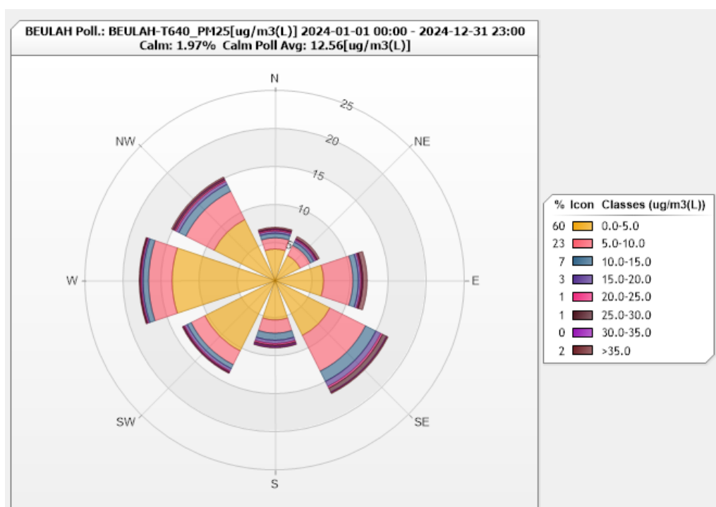
Figure 25. Beulah PM 2.5 Pollution Rose for 2024
