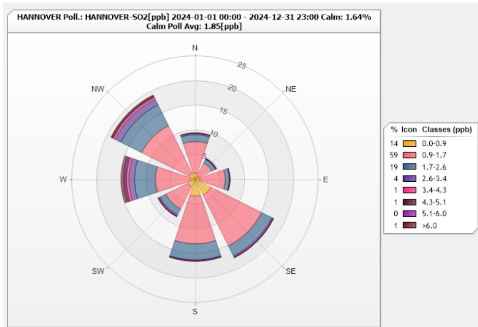
Figure 48. Hannover SO 2 Pollution Rose for 2024
