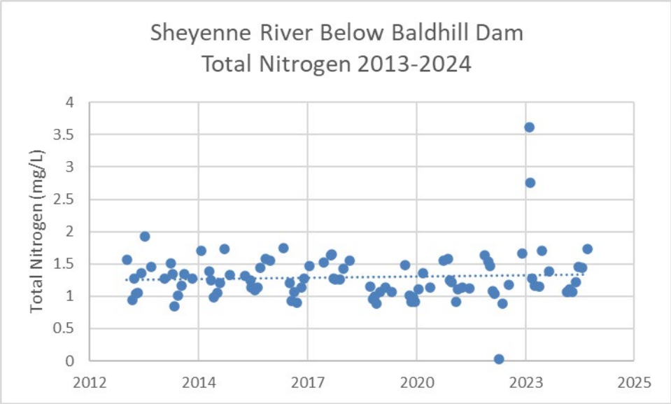
At the Sheyenne River below Baldhill Dam, Total Nitrogen concentrations have a slightly increasing trend, 2013-2024.
