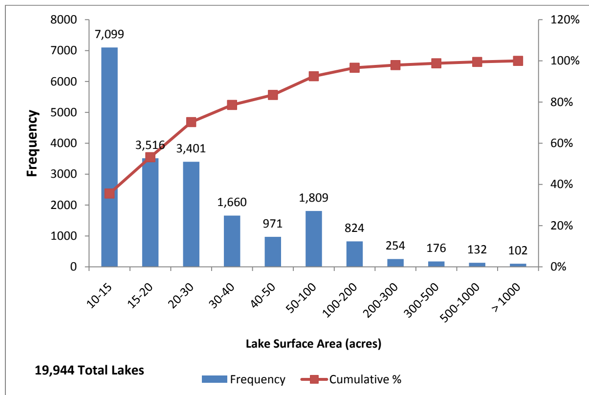
Figure 1a: Histogram of Study Area Lakes
