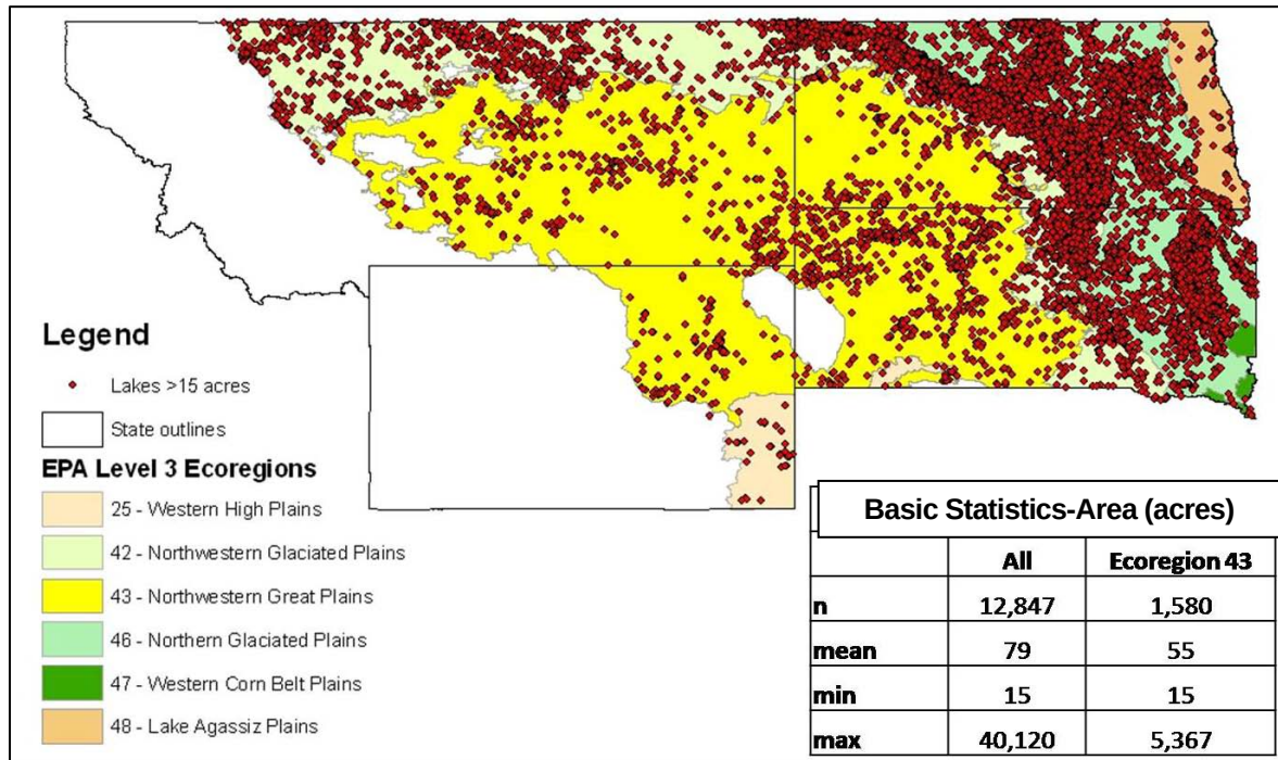
Figure 4a: Contents of the Lakes Master Database using Criteria of Lakes >15 acres
