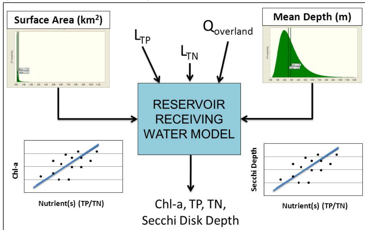
Figure 5: Structure of Reservoir Receiving Water Model
