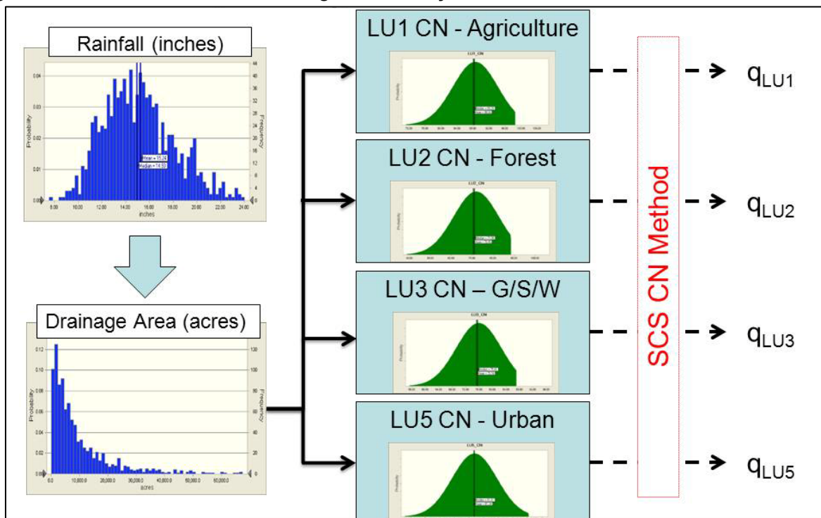
Figure 3: Structure of Watershed Loading Model – Daily Runoff Calculation
