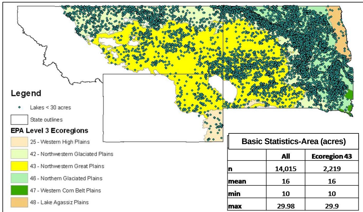
Figure 7a: Master Database Lakes that are <30 acres
