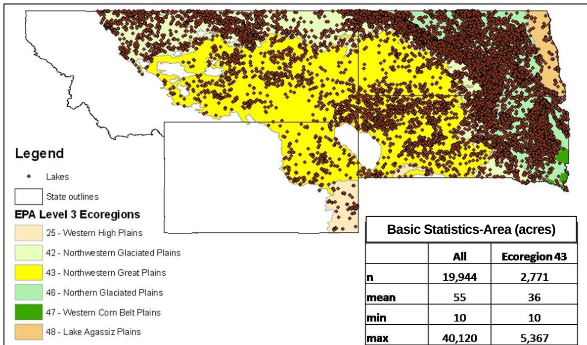
Figure 3a: Contents of the Lakes Master Database (Lakes >10 acres)
