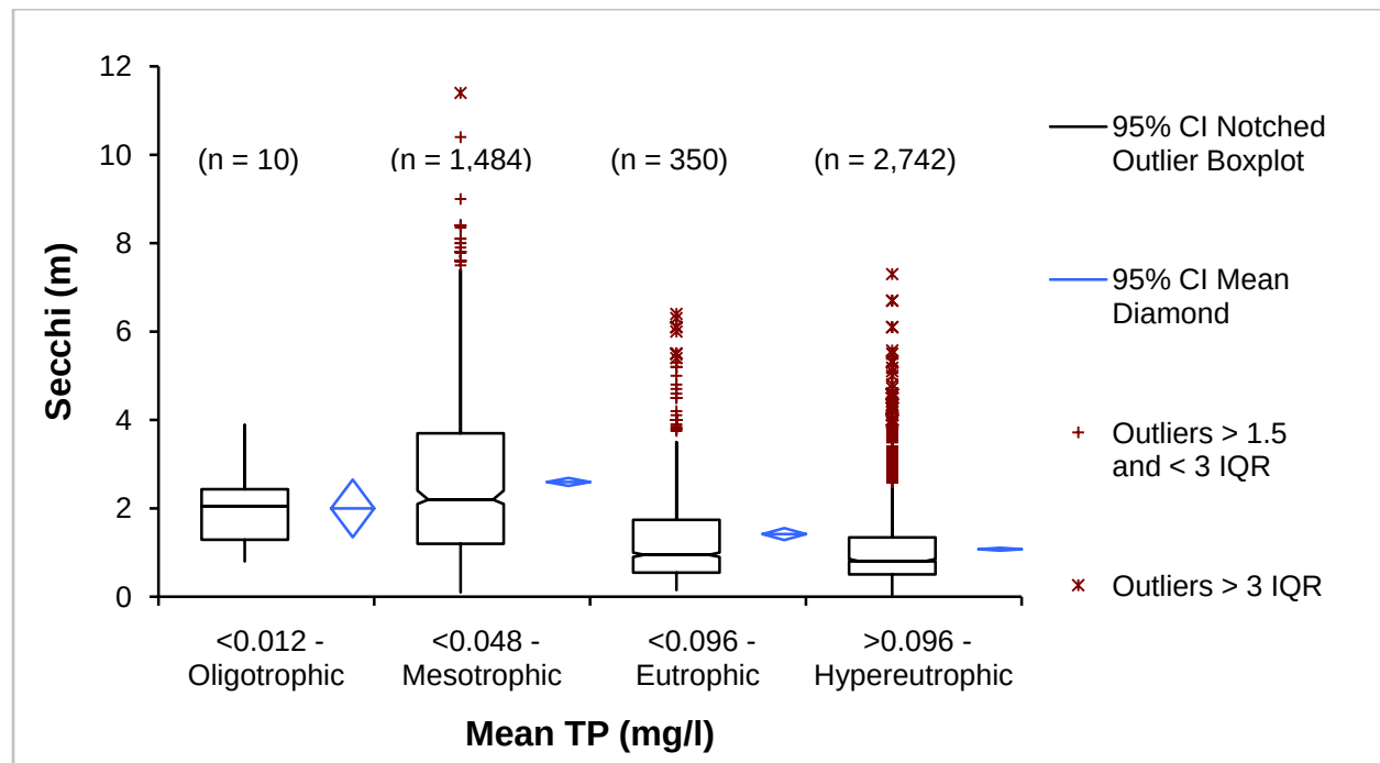
Figure 15: Distribution of Secchi Depth by Mean Reservoir TP – All Data
