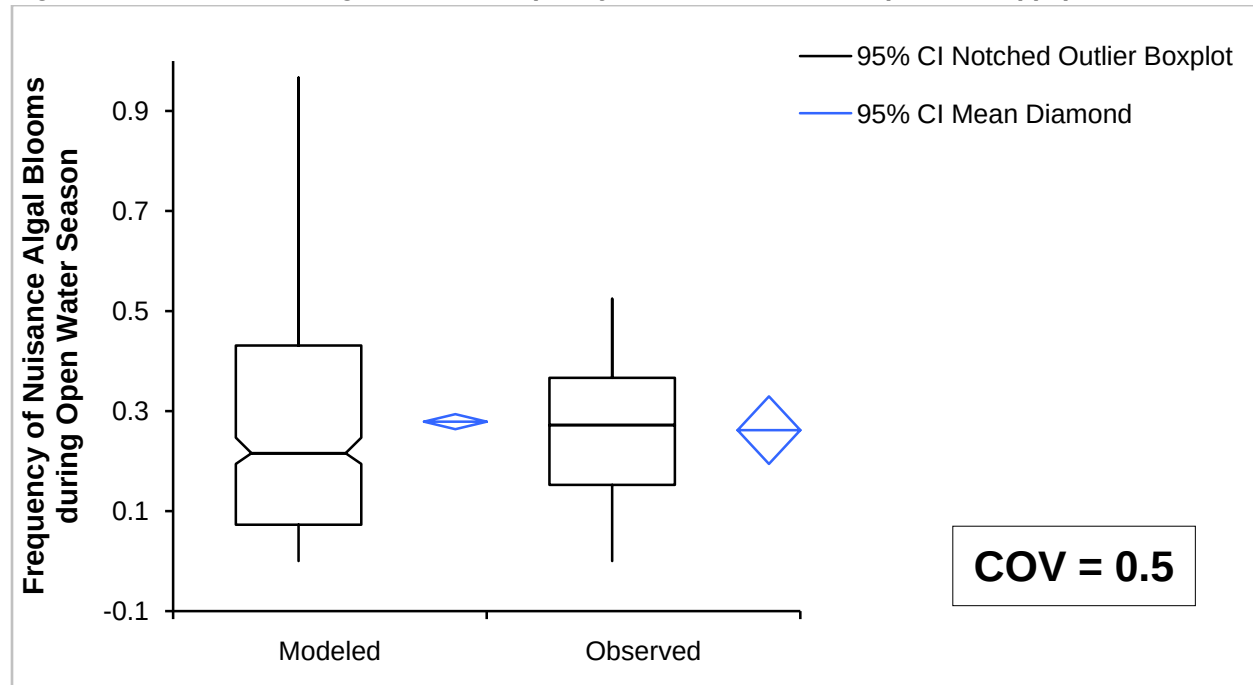
Figure 31: Results of Ecoregions 42/43 Frequency of “Nuisance” Bloom (Chl-a > 20 ppb) Estimation
