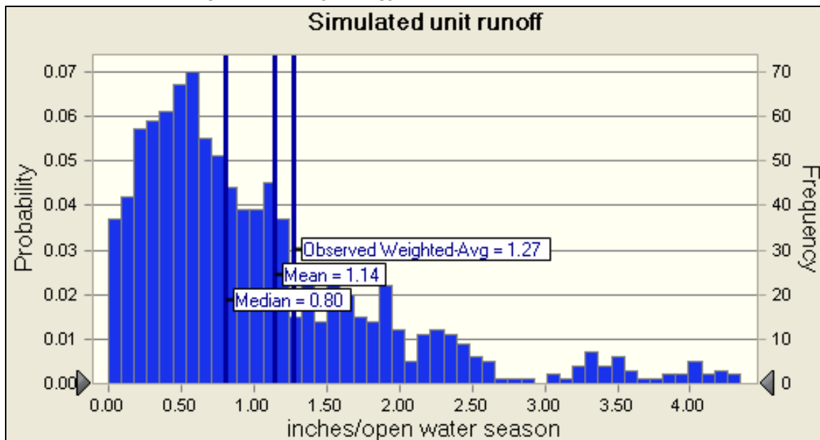
Figure 16: Results of Ecoregions 42/43 Hydrology Calibration
