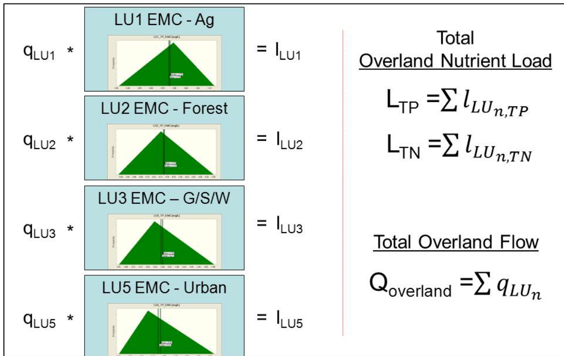
Figure 4: Structure of Watershed Loading Model – Pollutant Loading and Open Water Season Runoff and Loading Calculations
