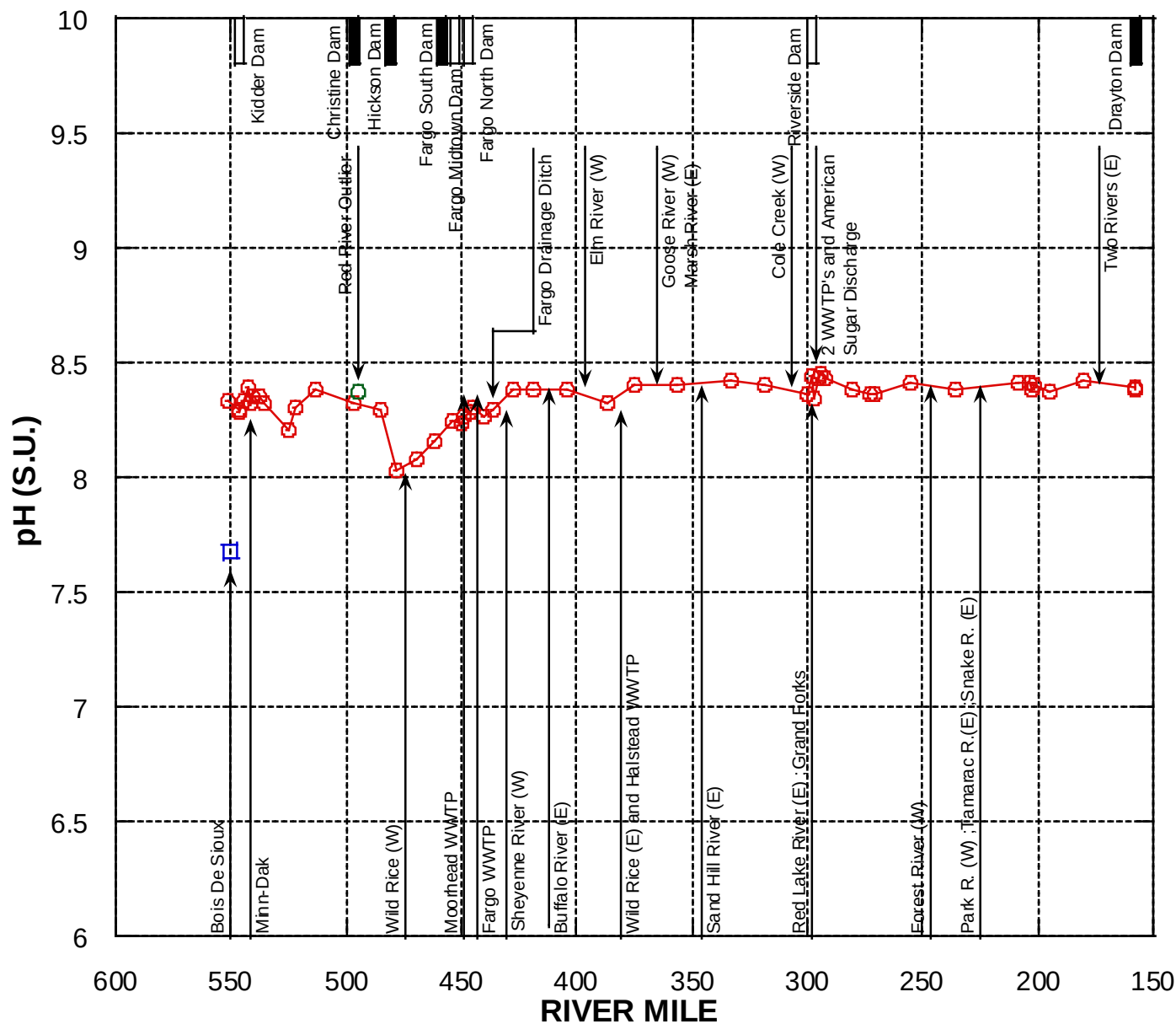
Figure 7. pH (S.U.) values at all 54 locations in the Red River mainstem between Wahpeton and Pembina, ND during the period August 18-September 1, 2010.
