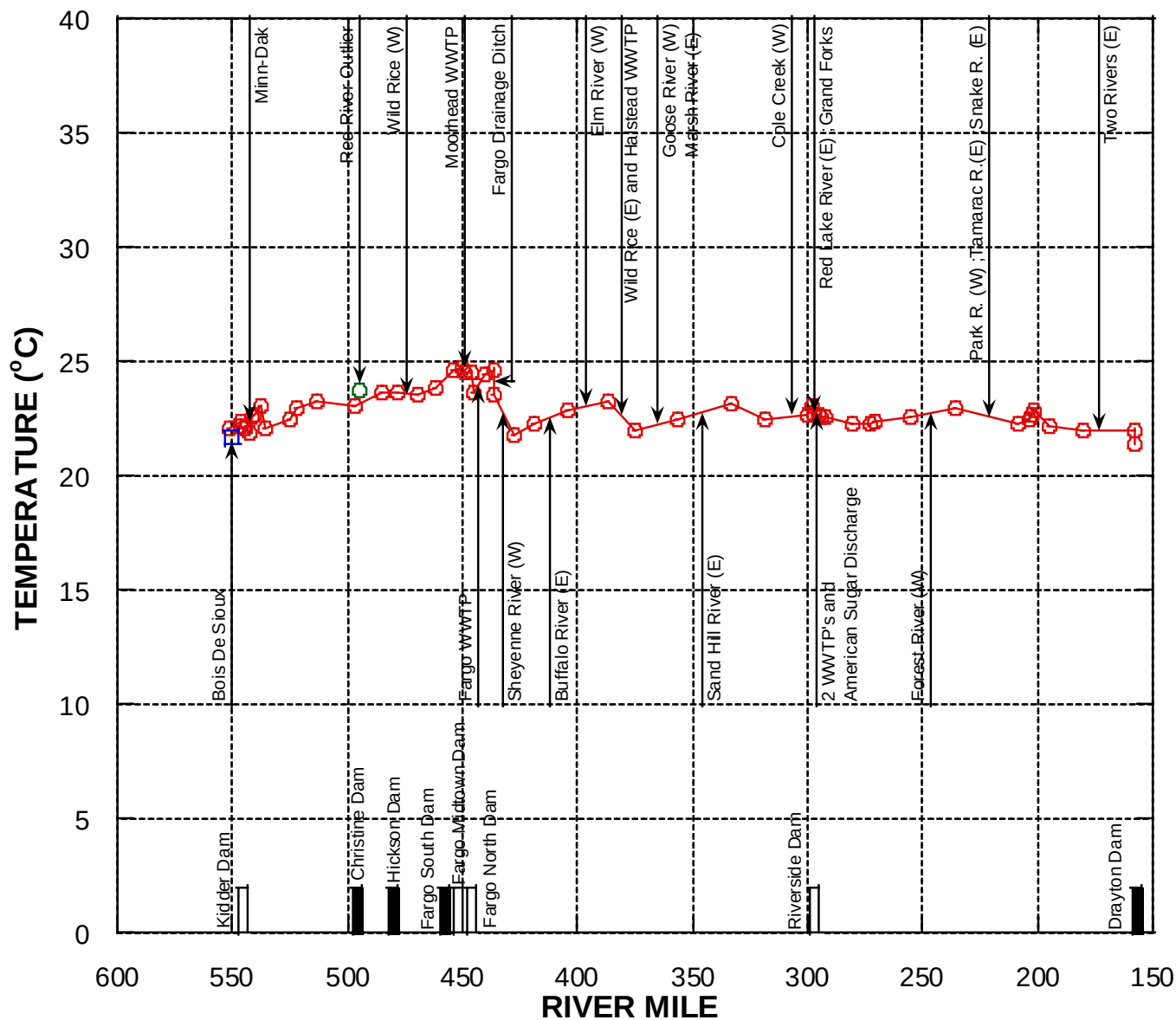
Figure 5. Temperature (°C) values at all 54 locations in the Red River mainstem between Wahpeton and Pembina, ND during the period August 18-September 1, 2010.
