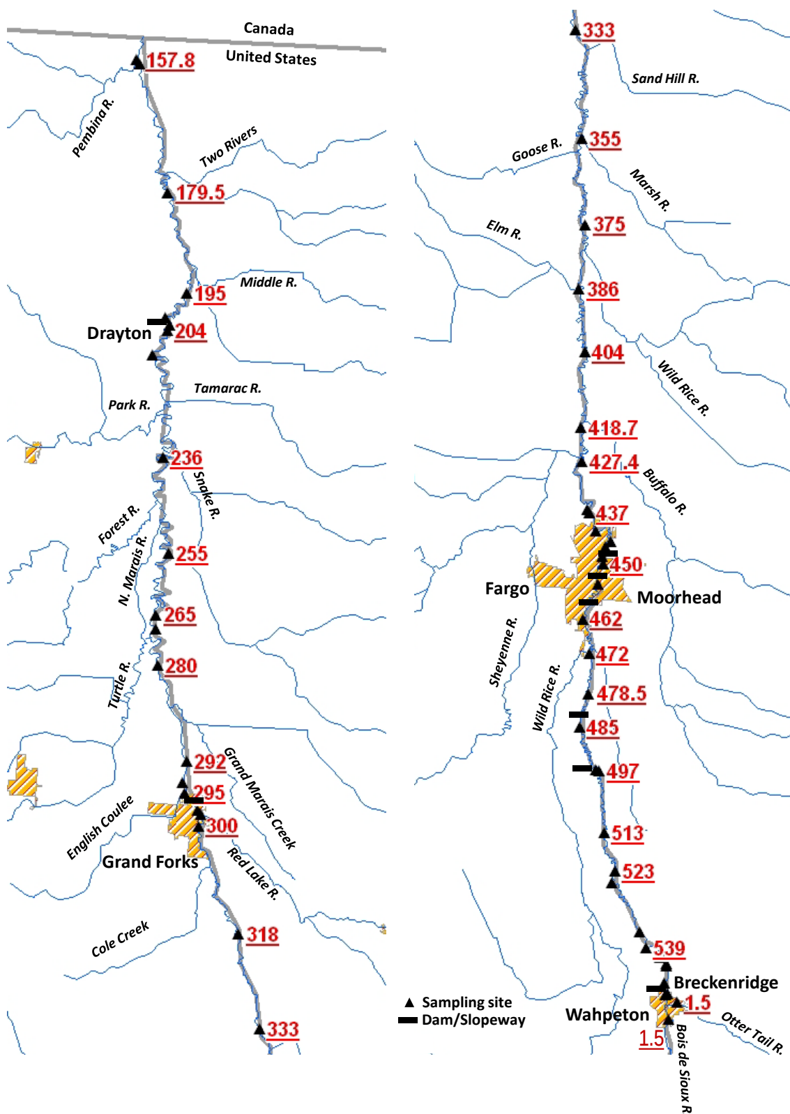
Figure 2. Red River of the North 2010 study area showing sampling locations (by river mile), major metropolitan areas, tributaries, and dams.
