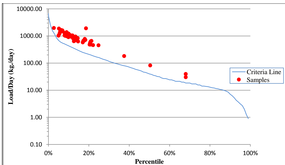
Figure 9. Total Nitrogen Load Duration Curve for the Sheyenne River Monitoring Station 385345 (The curve reflects flow data from 1990- 2010).
