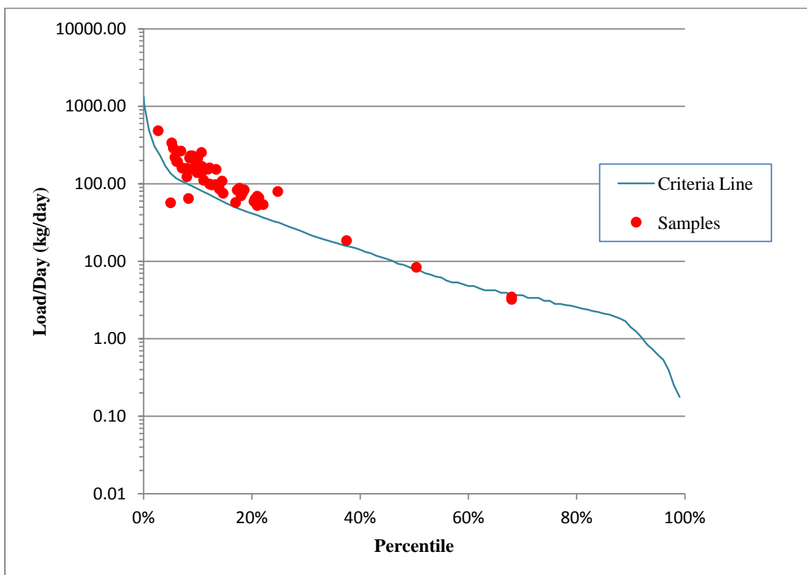
Figure 10. Total Phosphorus Load Duration Curve for the Sheyenne River Monitoring Station 385345 (The curve reflects flow data from 1990-2010).
