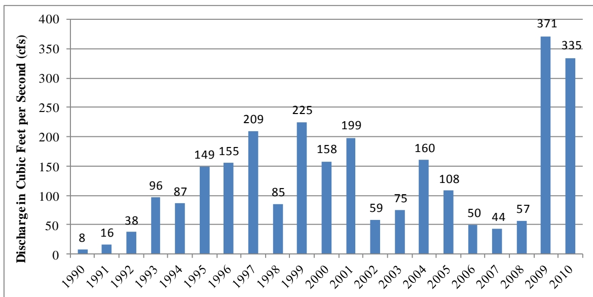
Figure 7. Mean Annual Discharge at the USGS Gauging Station (05056000) on the Sheyenne River near Warwick, ND.
