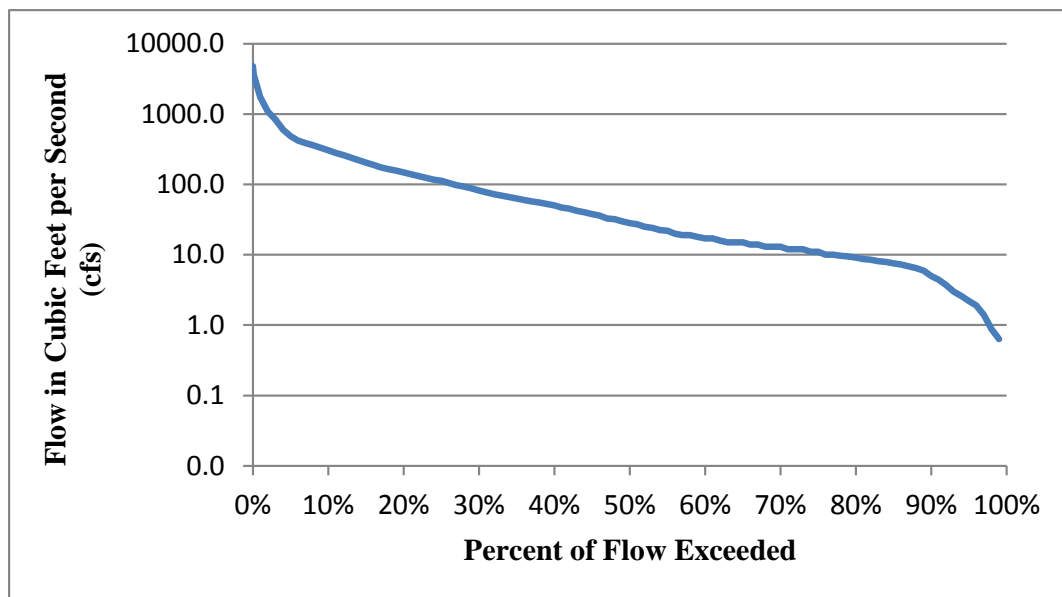
Figure 8. Flow Duration Curve for USGS Gauging Station 05056000.
