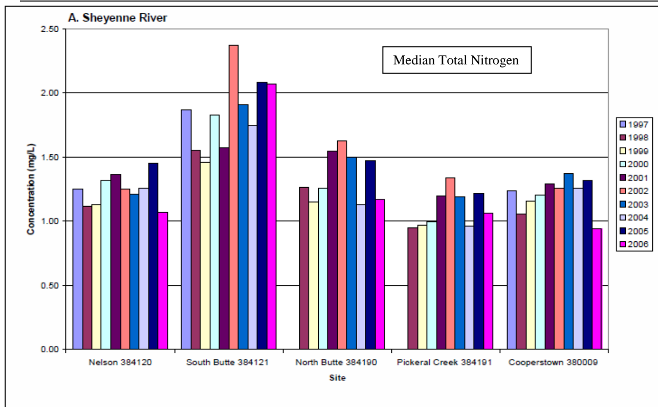
Figure 17. Median Total Nitrogen Concentrations for Sites Along Sheyenne River, 1997-2006.
