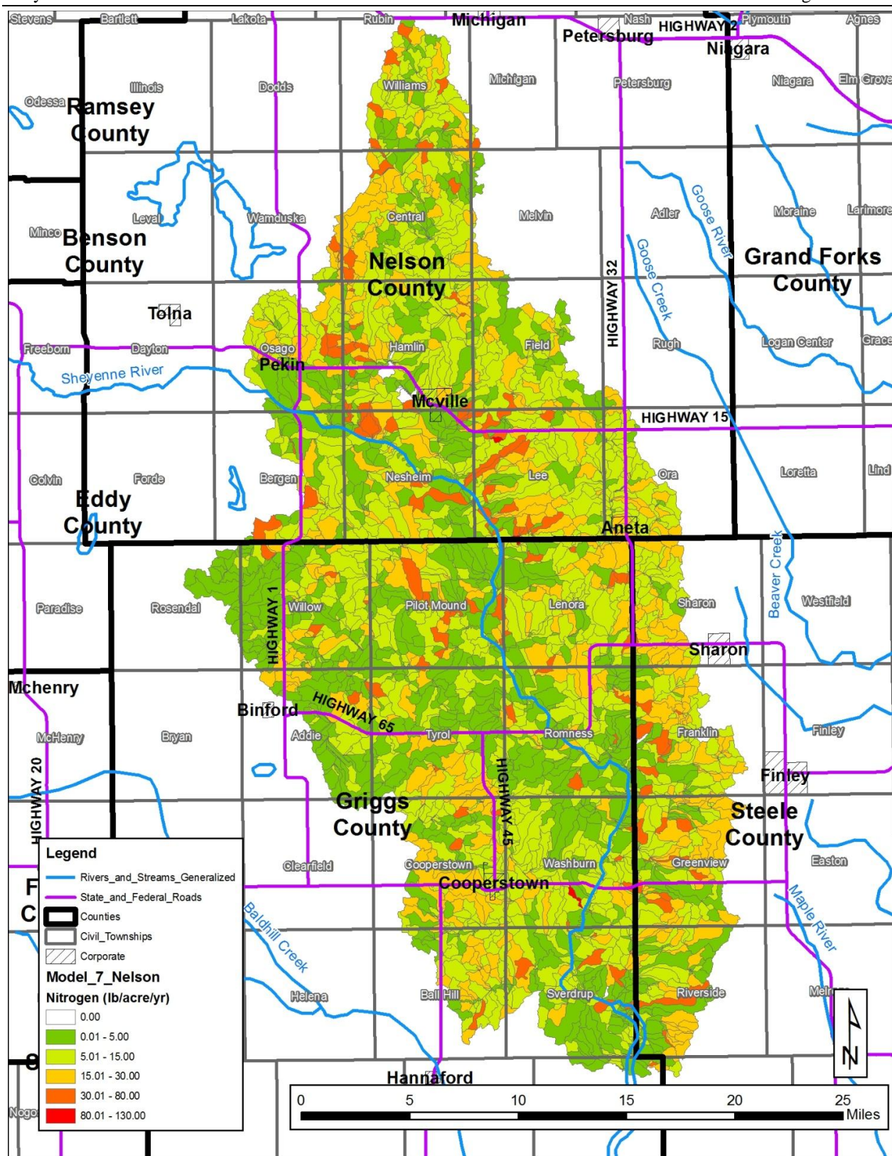
Figure 24. AnnAGNPS Model Predicted Nitrogen Yield for the Nelson Model (Moore Engineering, 2010).
