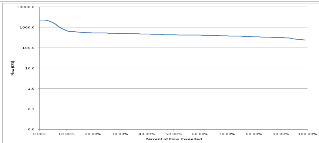
Figure 9. Flow Duration Curve for 473842098071001 (Monitoring Station 384120).
