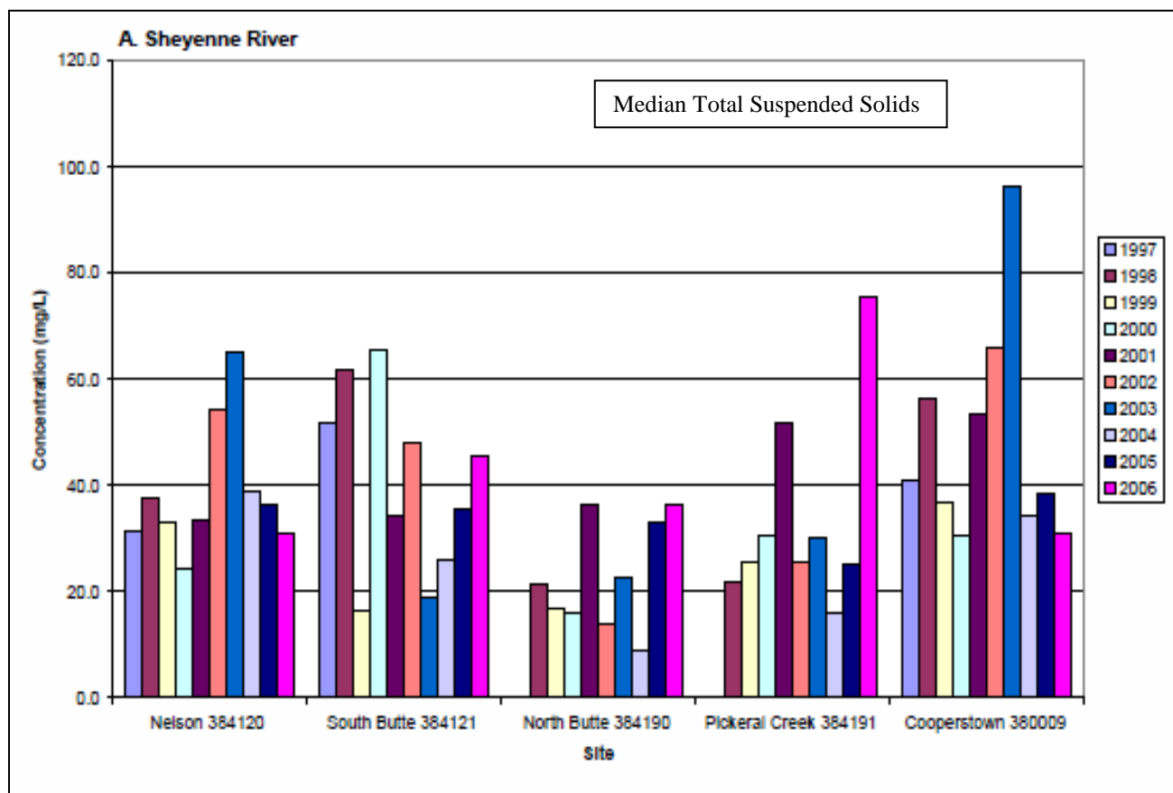
Figure 19. Median Total Suspended Solids Concentrations for Sites Along Sheyenne River, 1997-2006.
