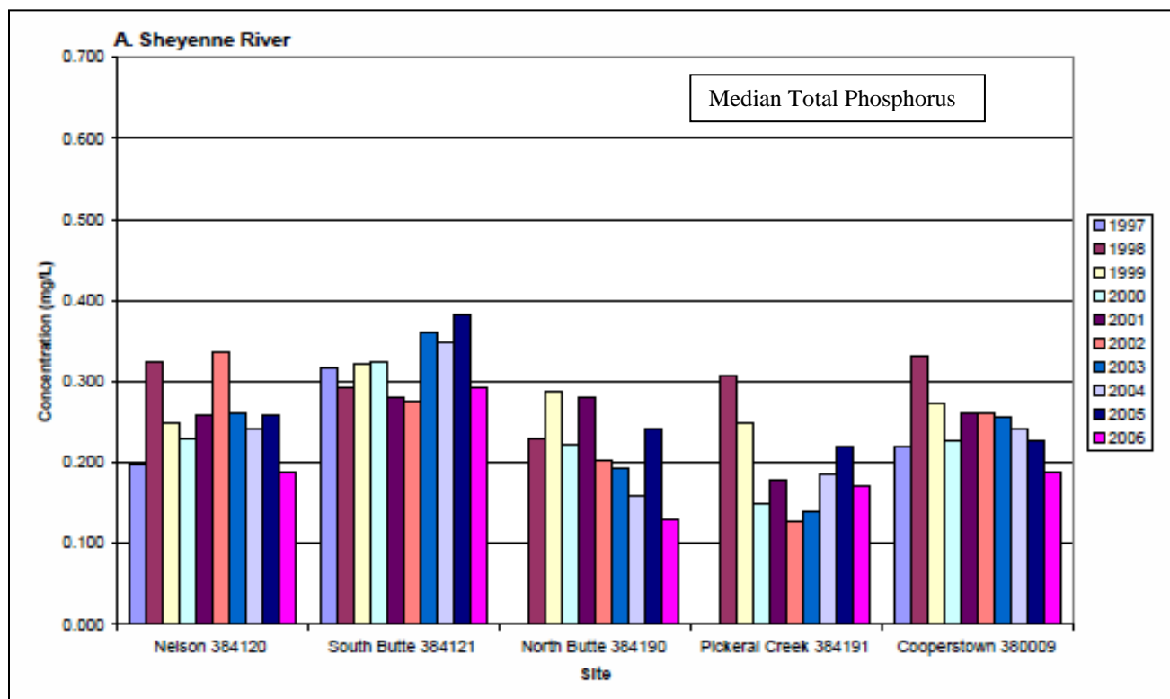
Figure 18. Median Total Phosphorus Concentrations for Sites Along Sheyenne River, 1997-2006.
