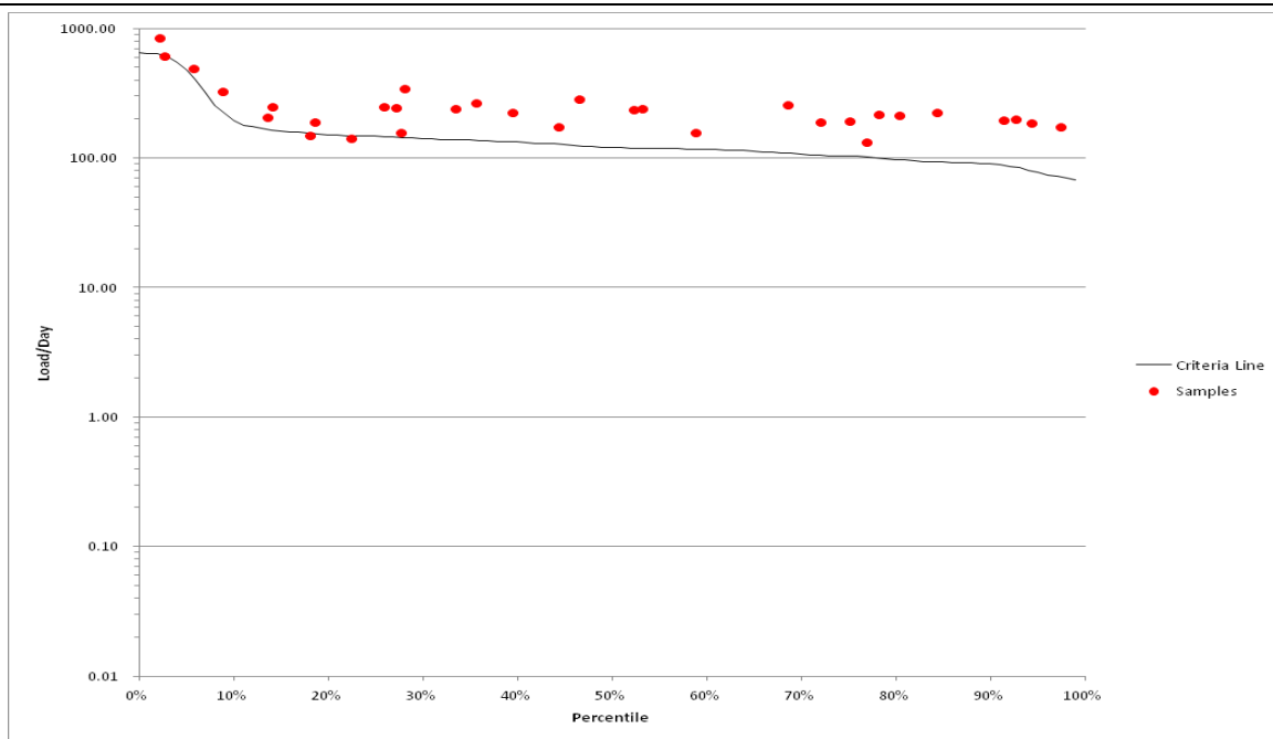
Figure 13. Total Phosphorus Load Duration Curve for the Sheyenne River Monitoring Station 384120 (The curve reflects flow data from 2010).
