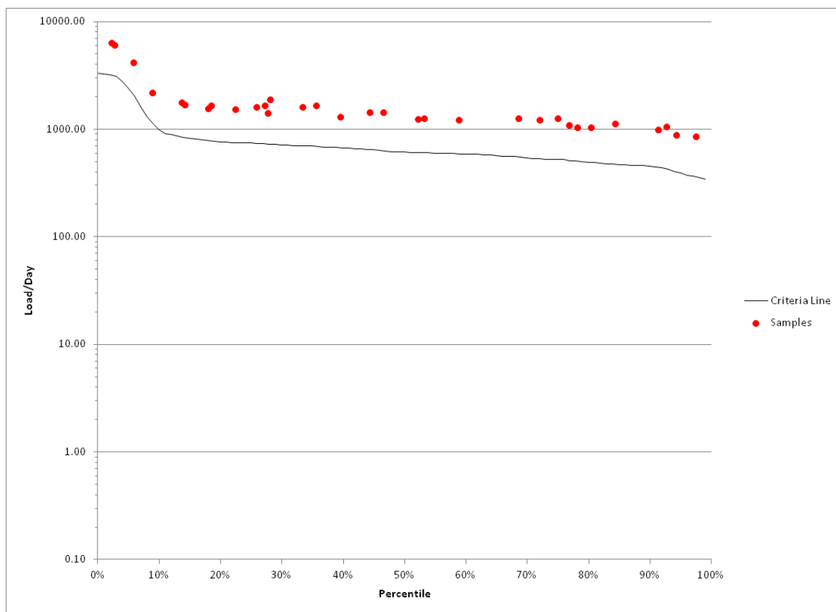
Figure 11. Total Nitrogen Load Duration Curve for the Sheyenne River Monitoring Station 384120 (The curve reflects flow data from 2010).
