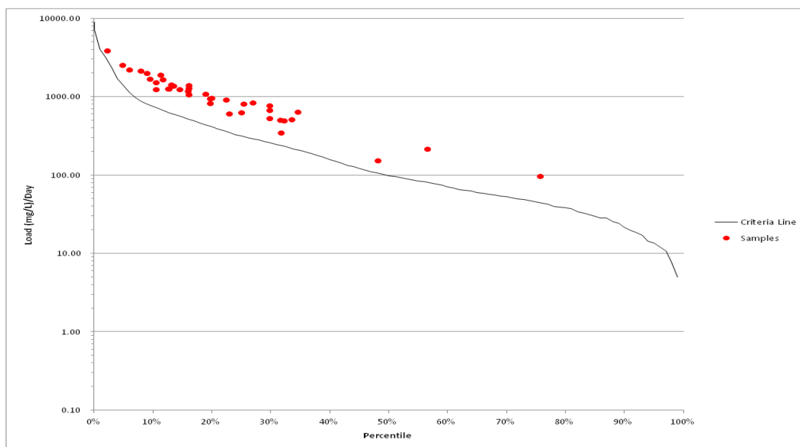
Figure 10. Total Nitrogen Load Duration Curve for the Sheyenne River Monitoring Station 380009 (The curve reflects flow data from 1990-2010).
