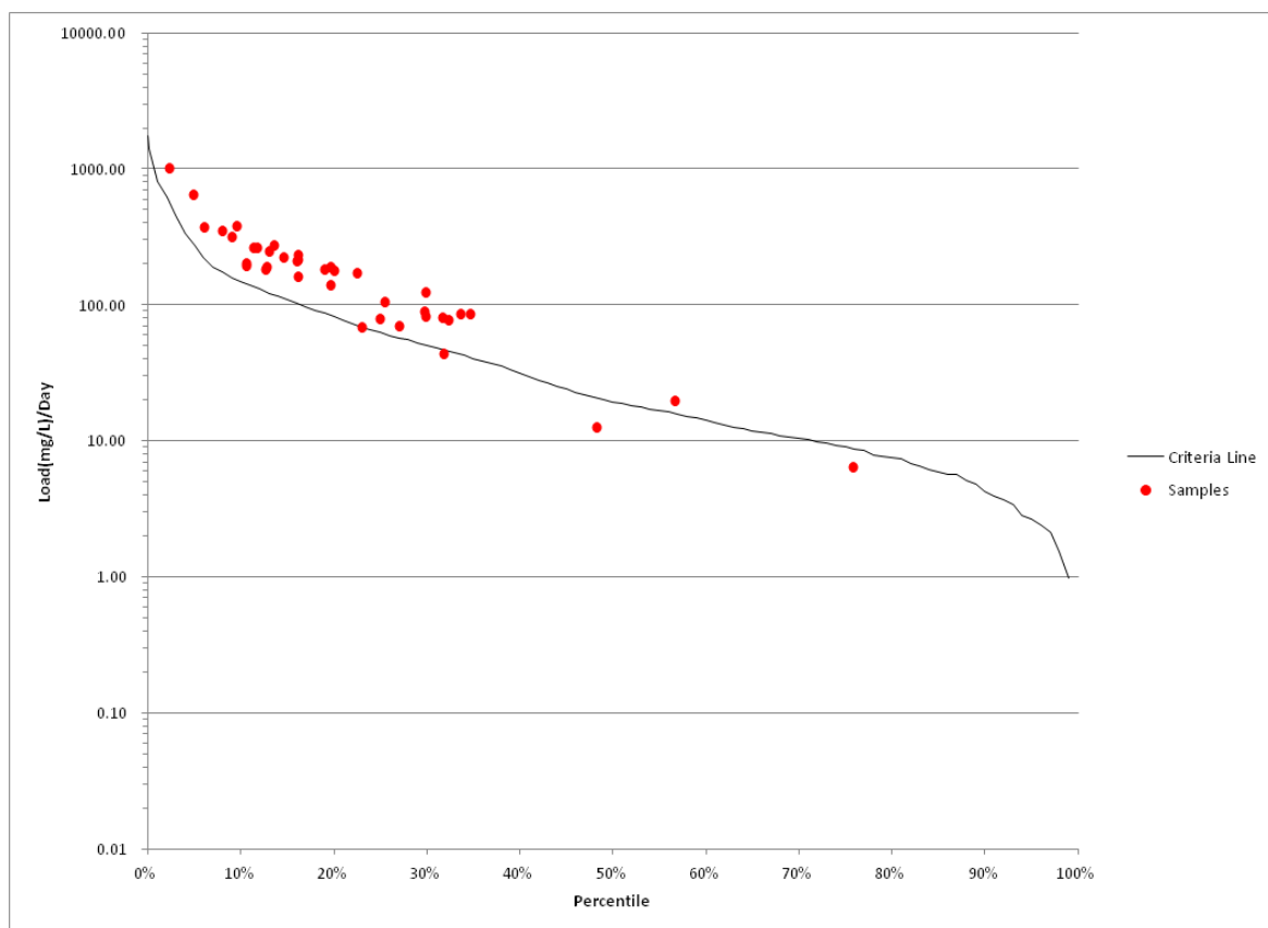
Figure 12. Total Phosphorus Load Duration Curve for the Sheyenne River Monitoring Station 380009 (The curve reflects flow data from 1990-2010).
