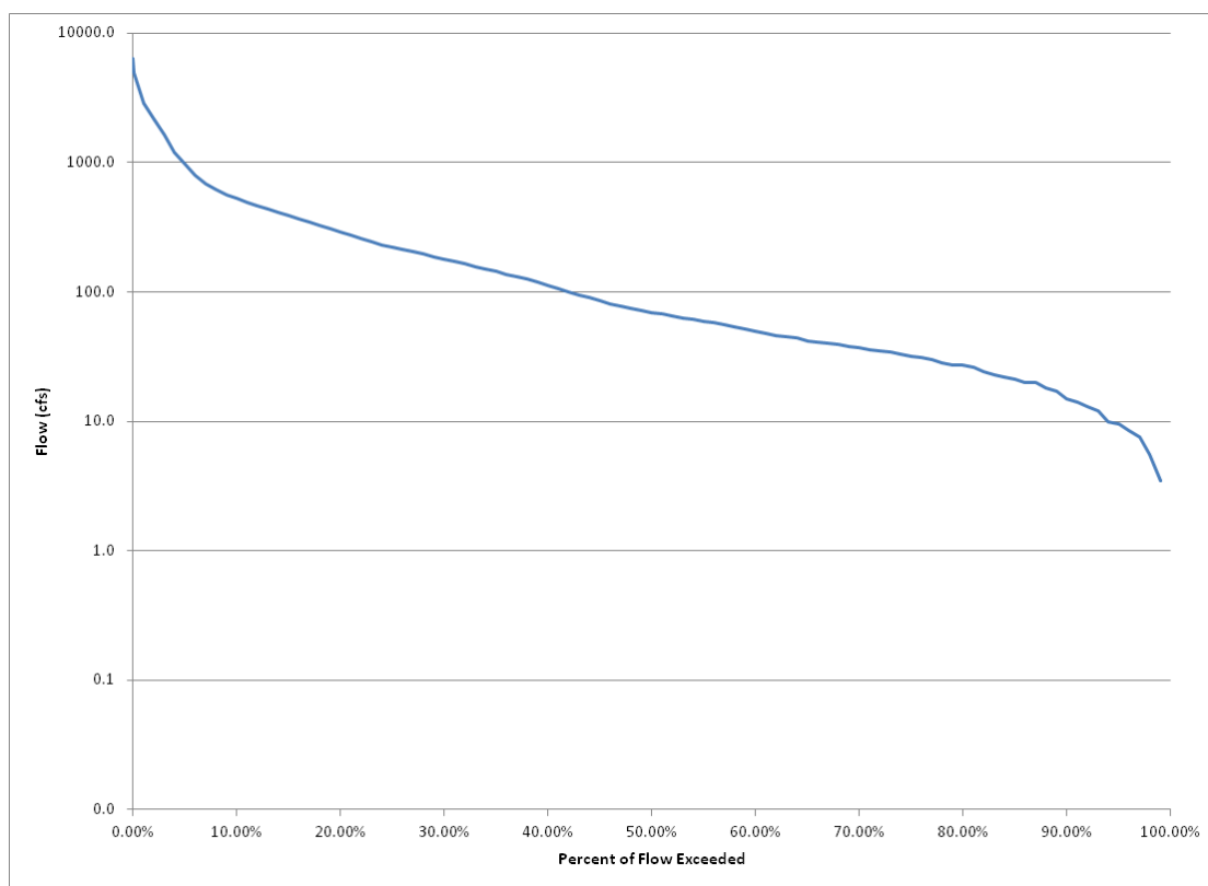
Figure 8. Flow Duration Curve for USGS Gauging Station 05057000 (Monitoring Site 380009).
