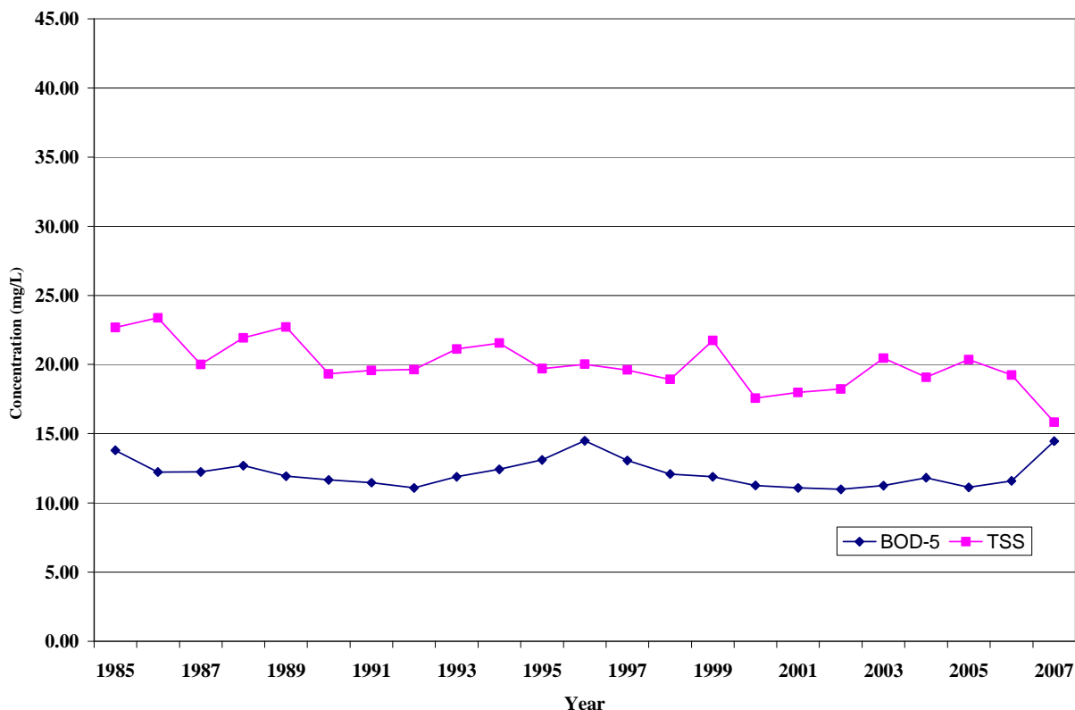
Figure III-2. Average Annual BOD-5 day and TSS Concentrations for Wastewater Discharges in North Dakota (1985-2007)
