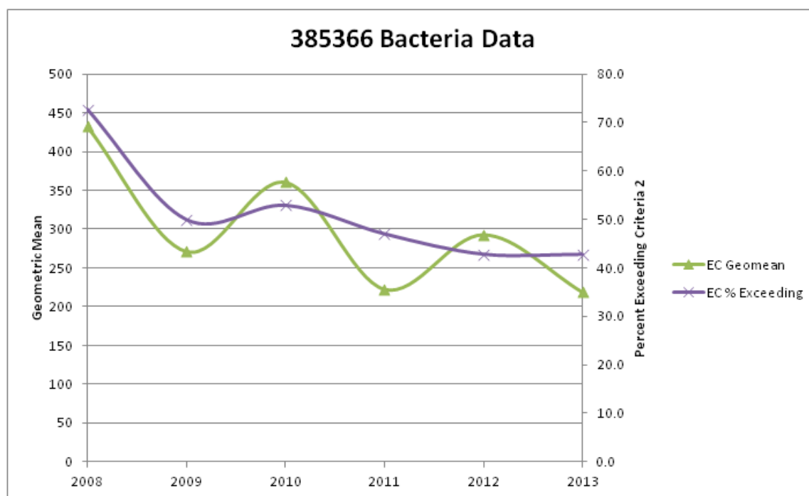
Figure III-6. E. coli Bacteria Annual (May-September) Geometric Mean Concentrations and the Percentage of Samples Exceeding the 409 CFU/100mL Water Quality Standard for Seven Mile Coulee Site 385366.
