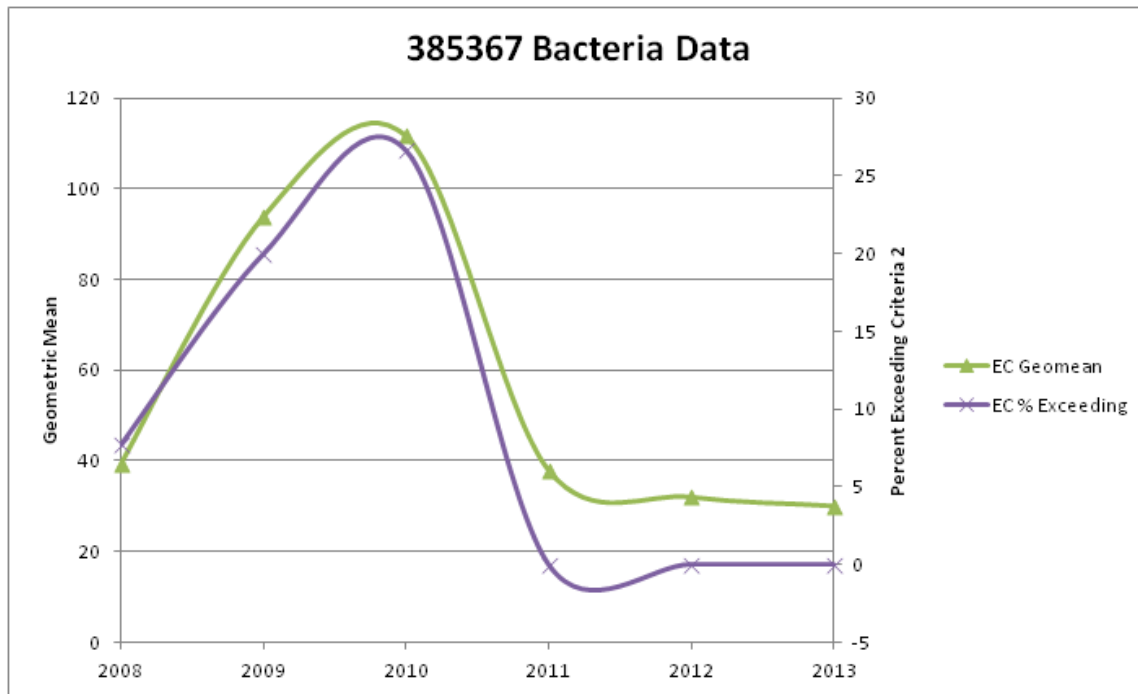
Figure III-7. E. coli Bacteria Annual (May-September) Geometric Mean Concentrations and the Percentage of Samples Exceeding the 409 CFU/100mL Water Quality Standard for Seven Mile Coulee Site 385367.
